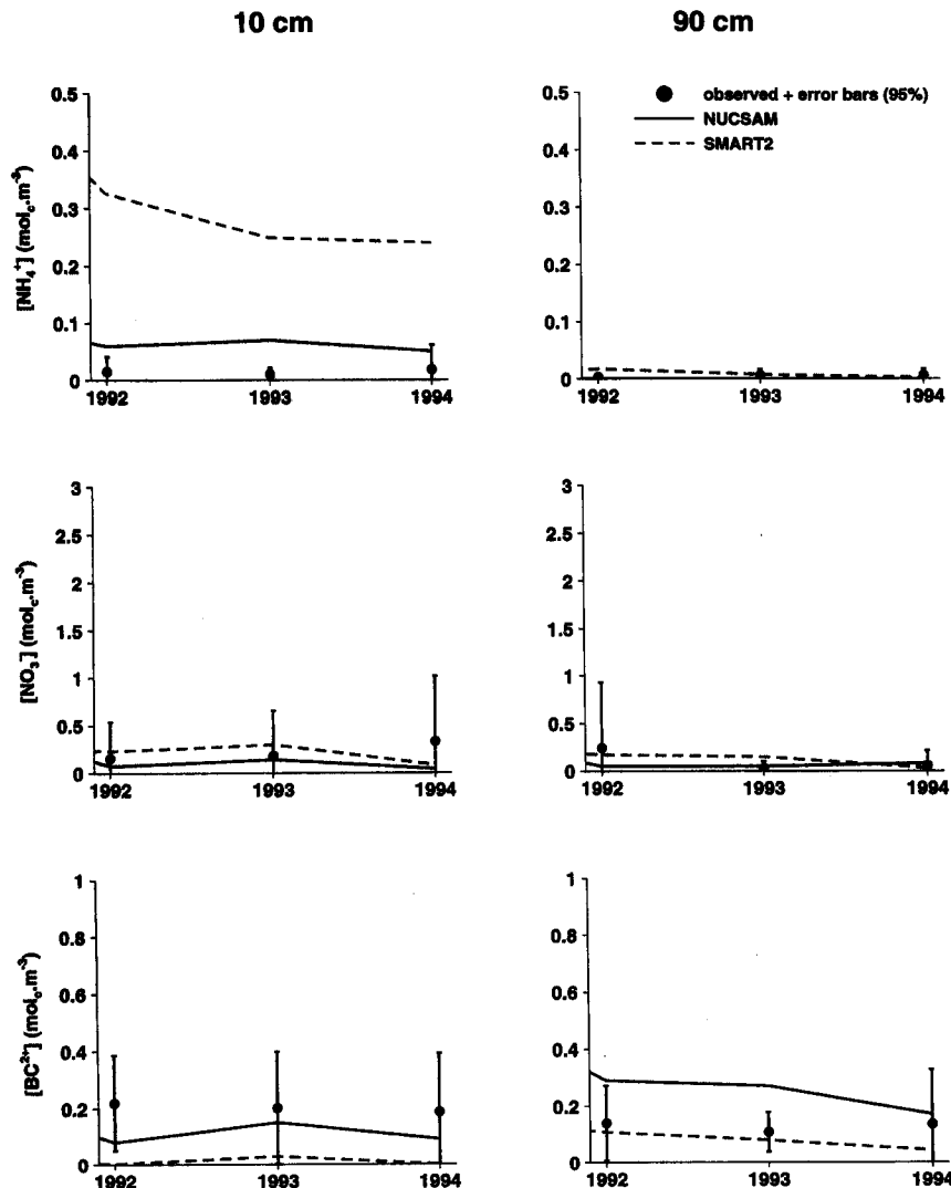
Fig. 3. Simulated and observed flux-weighted annual average concentrations of NH_4^+ , NO_3^- and BC^{2+} ( Ca^{2+} + Mg^{2+} ) at 10 cm and 90 cm depth for the pristine plot. For the observations the error bars of the 95% confidence interval are included.
