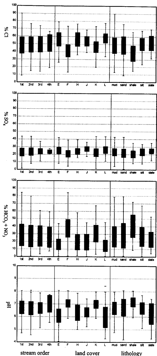
Fig. 8. Box and whisker diagrams of anionic composition and pH based on sub-classes of Lower Silurian streamwaters.
