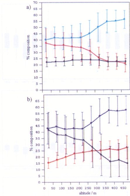
Fig. 3. Differences in Lower Silurian streamwater composition with altitude; (a) cations, (b) anions.
