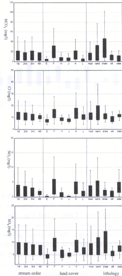
Fig. 6. Box and whisker diagrams of anion concentration based on sub-classes of Lower Silurian streamwaters.
