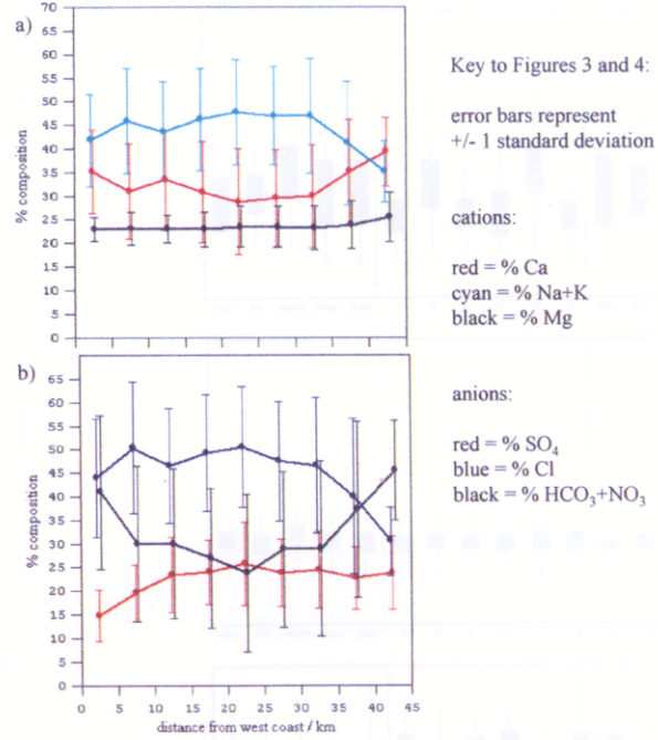
Fig. 4. Differences in Lower Silurian streamwater composition with coastal proximity; (a) cations, (b) anions.
