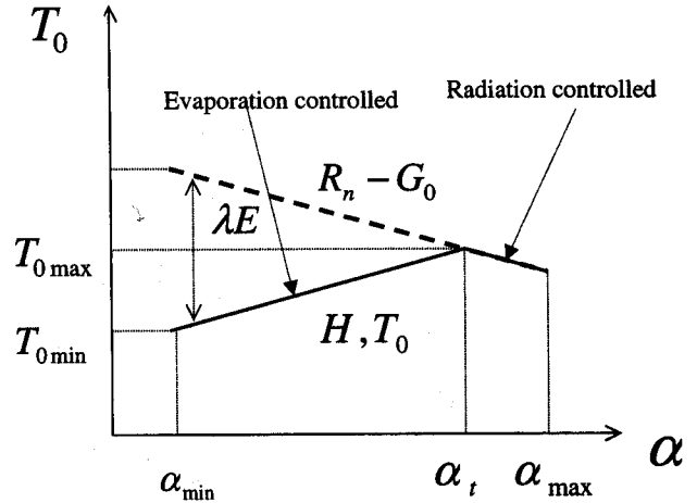
Fig. 3. Schematic representation of the relationship between surface reflectance and temperature: The solid line denotes the relationship between temperature (and also sensible heat) and reflectance, while the dashed line represents the relationship between available energy and reflectance. The difference between the dashed and the solid line gives the latent heat flux according to the energy balance.
