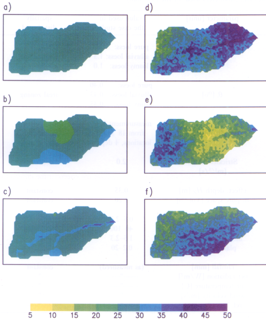
Fig. 5. Initial soil moisture values (in Vol-%, averaged over the depth 0–60 cm) at July 13, 1992, subcatchment Neuenbürger Pfad, obtained by different methods: a) area averaged value; b) by the OK method; c) by the MBU method; d)–f) three realisations of the simulation technique.
