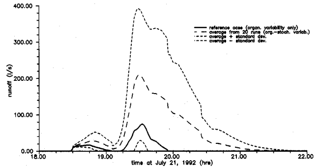
Fig. 7. Simulated hydrographs and their standard deviation from subcatchment Neuenbürger Pfad, obtained by using organised and 20 realisations of organised/stochastic initial soil moisture fields (storm event of July 21, 1992)
