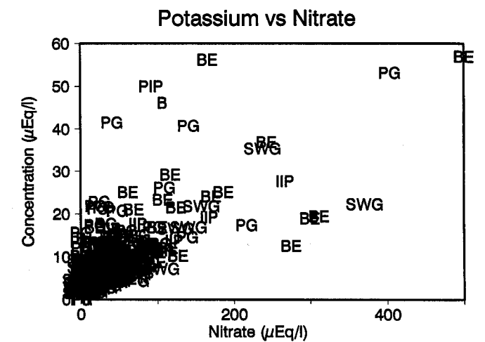
Fig. 8. Plots of the concentrations of calcium, barium and potassium against nitrate.
