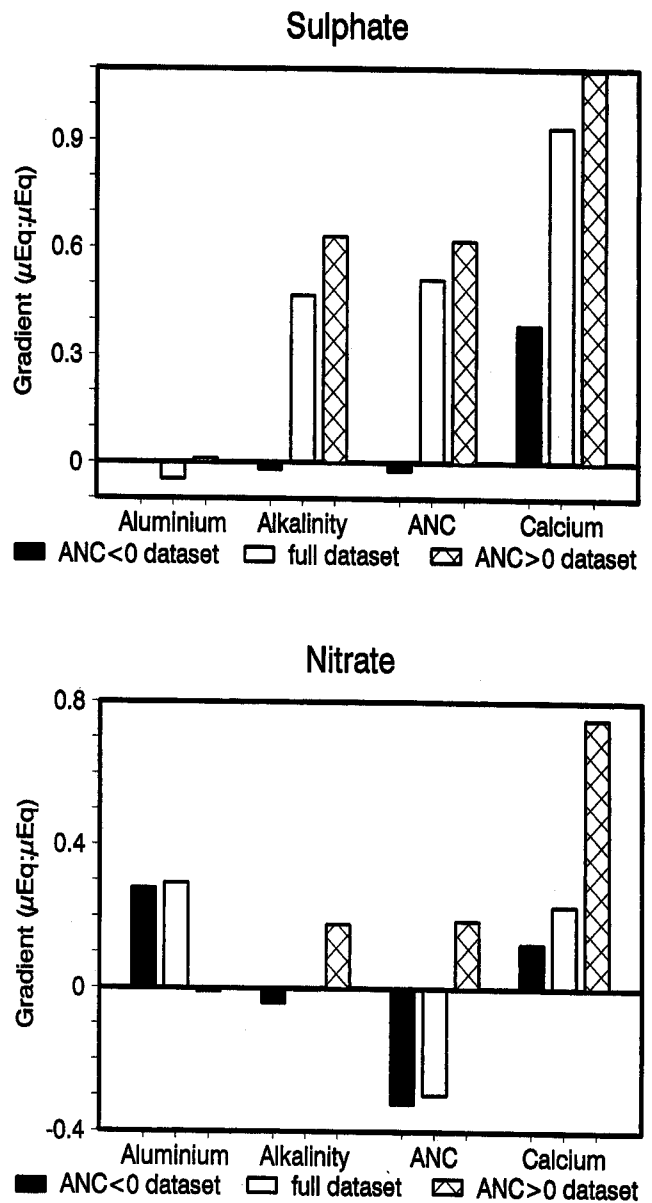
Fig. 10. Plots of average regression coefficients for aluminium, alkalinity, ANC and calcium against sulphate and nitrate.
