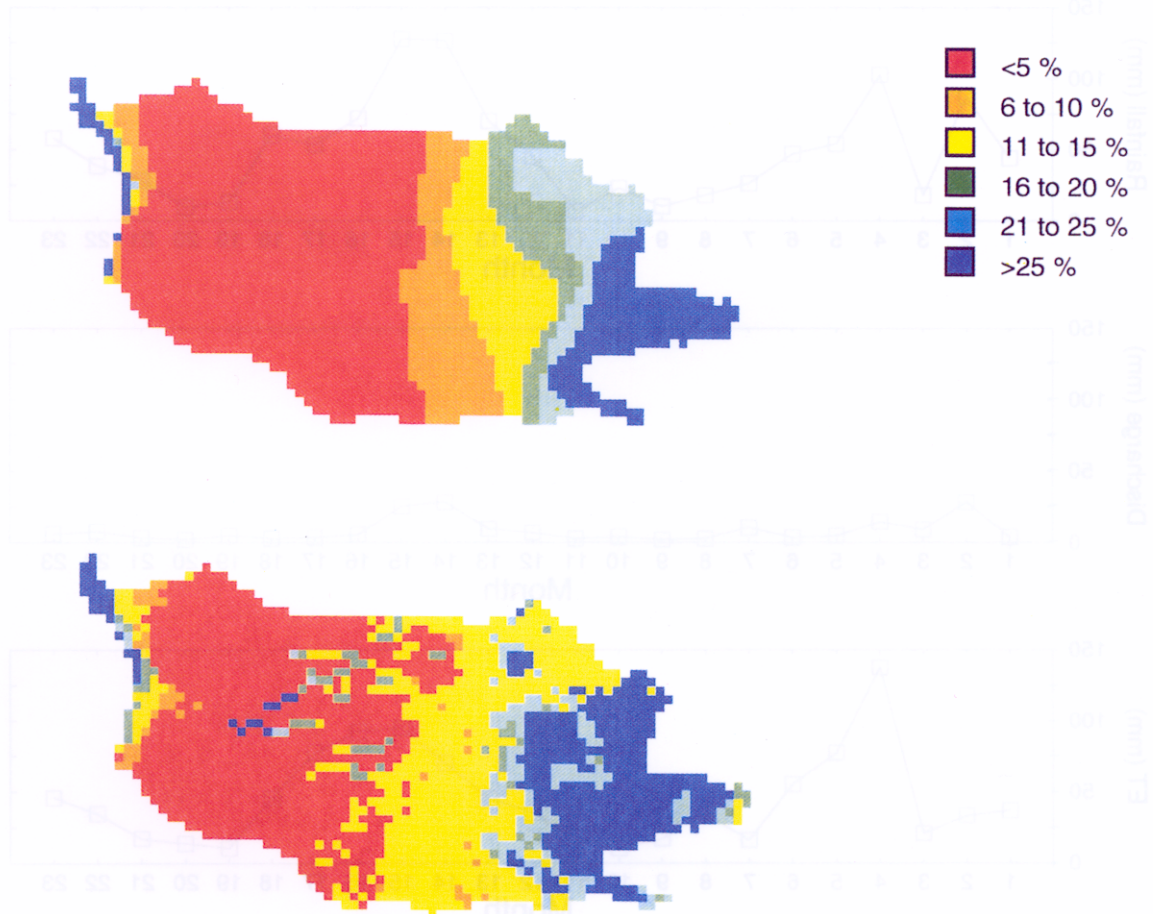
Fig. 9. Annual mean ratio of runoff to precipitation: comparison of simulated (July 1994–May 1996, lower panel) and long term mean (1951–1980, upper panel) observed values.
