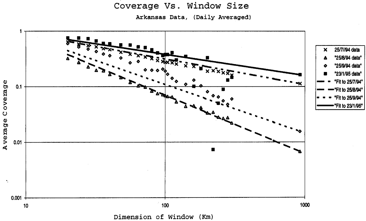
Fig. 4. Rainfall coverage as a function of window size.
