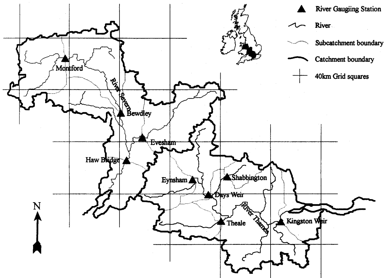
Fig. 1. Severn and Thames catchments.
