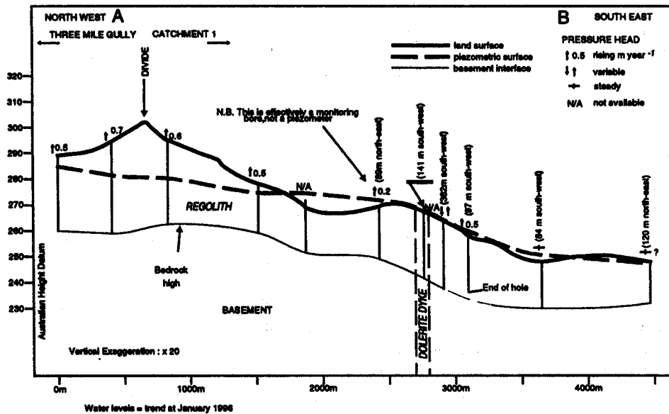
Fig. 6. Longitudinal section A-B along Catchment 1. See Fig. 3 for location of section.
