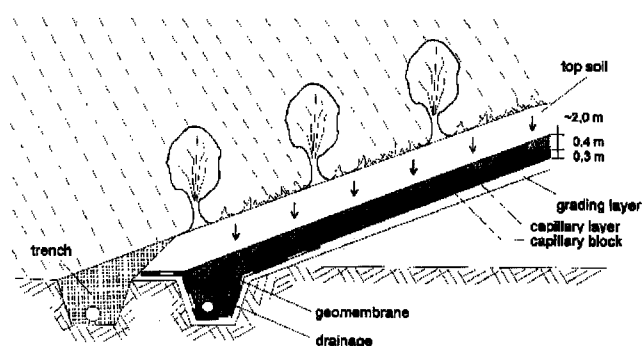
Fig. 1. Landfill cover system with a capillary barrier.
