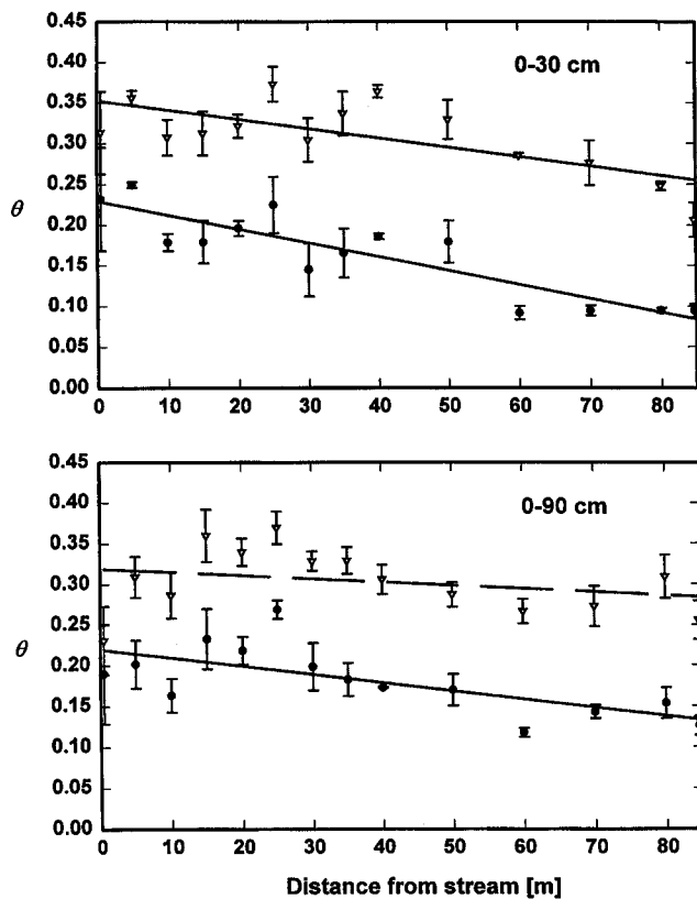
Fig. 2. Soil moisture response ranges: from drought (11 November, 1991; \bullet -) through 24.3 cm precipitation recharge (2 December, 1991; \dashv -). Each point is a mean of 3 measurements. Least squares regressions of soil moisture content on distance along hillslope in the shallow layer showed significant ( p < .05 ) gradients before and after recharge. Regressions in the deeper layer showed a significant gradient during drought, but not after recharge.
