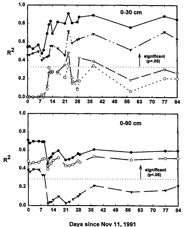
Fig. 3. Squared partial correlations for physiographic variables vs. soil moisture content during the measurement period. Physiographic variables shown are: topographic index ( \dashv -), soil storage index ( \circ -), and organic matter index ( \triangle -). Also shown are adjusted r^2 values for multiple regressions of physiographic variables on soil moisture ( \bullet -); only those variables that were significant in partial F tests ( p < .05 ) were included.
