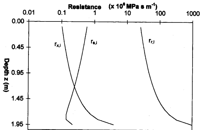
Fig. 4. Variation of soil, root and xylem elementary resistances r_{s,i} , r_{r,i} and r_{x,i} as a function of depth in the conditions corresponding to case 4.
