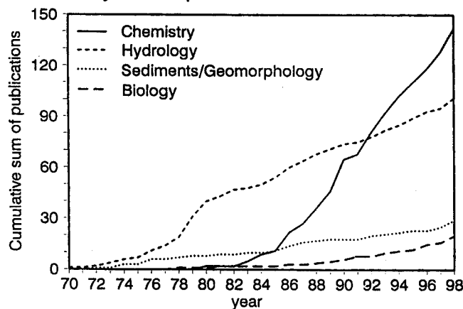
Figure 1. Graphs showing the publication record for the Plynlimon study over time for the main study disciplines of Hydrology, chemistry, biology and sedimentology/geomorphology.
