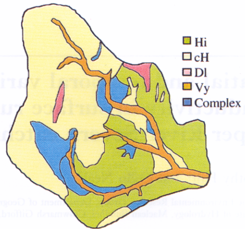
Fig. 3. Soil Map
