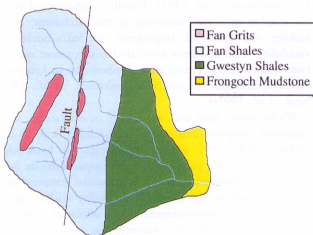
Fig. 2. Geological Map
