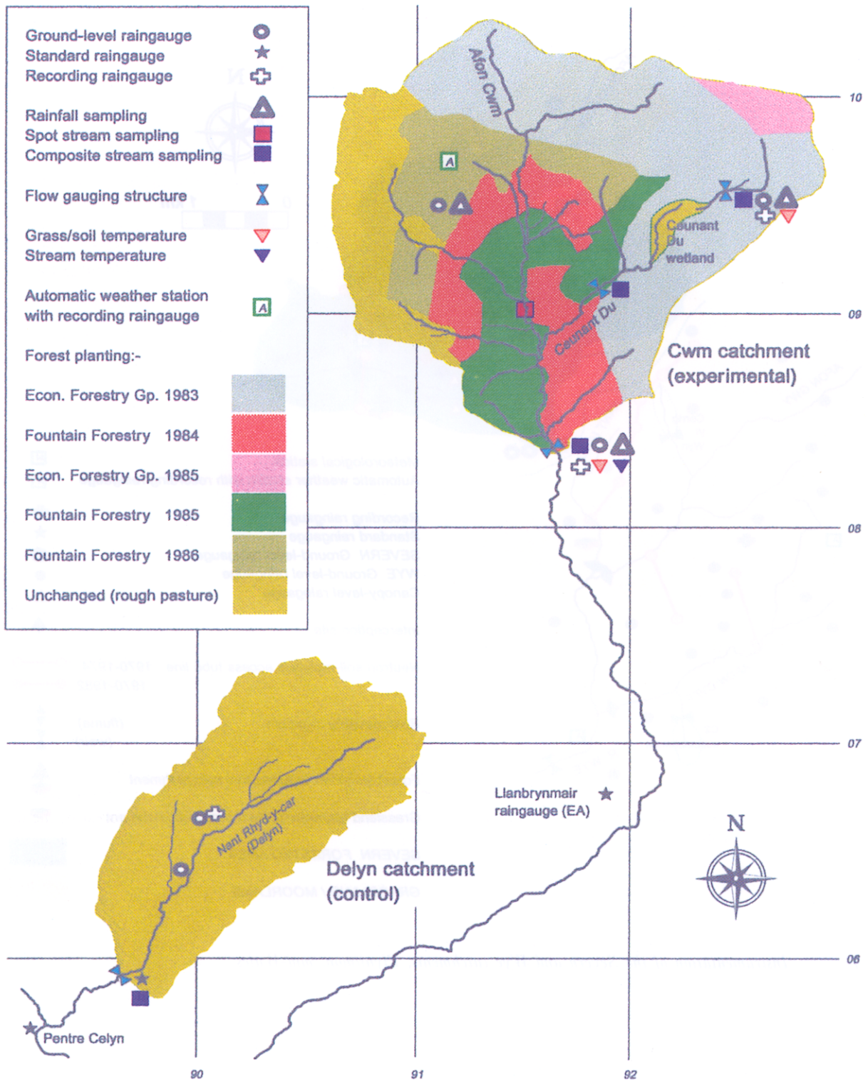
Plate 8 Instrumentation and forest history of the Llanbrynmair catchments, mid-Wales (see page 391)
