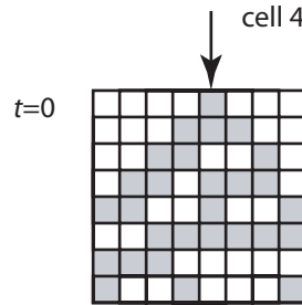
Fig. 4: Values taken by cell 4: 11011100.
