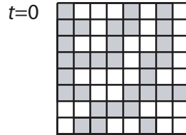
Fig. 3: Evolution of CA30 on a ring with N = 8 cells.
