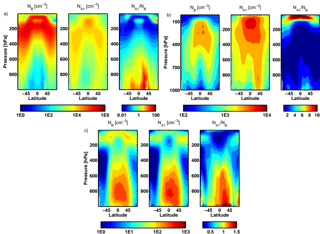
Fig. 2. Annual zonal average concentrations [cm -3 STP (1013.25 hPa, 273.15 K)] of (a) nucleation mode aerosol number; (b) sum of Aitken mode number concentration; and (c) sum of accumulation mode number concentration. Left panels show the Experiment B (standard ECHAM-HAM); centre ones Experiment A1 (using activation nucleation in addition to the standard binary nucleation); and right panels show the ratio of the yearly averages for Experiments B and A1. Notice the different color scales between figures.
