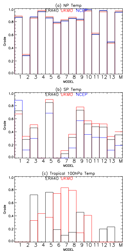
Fig. 5. Comparison of model grades for the (a) Temp-NP, (b) Temp-SP, and (c) Temp-Trop tests when ERA40 (black), UKMO (red), or NCEP (blue) meteorological analyses are used for the observations in the metric (4).
