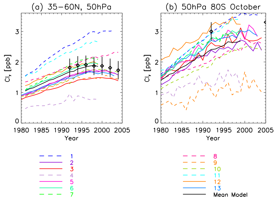
Fig. 1. Time series of (a) annual-mean, 35°–60° N, and (b) October-mean, 80° S Cl y at 50 hPa from CCM simulations (curves) and observations (symbols plus vertical bars).
