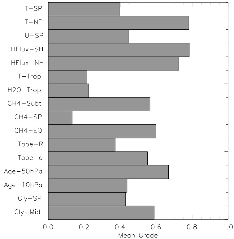
Fig. 3. Average grade over all models for each diagnostic test.
