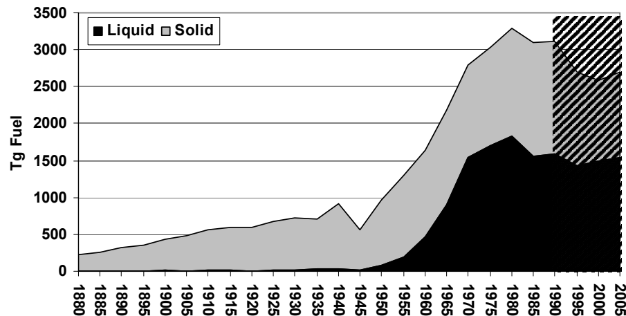
Fig. 3. European solid and liquid fossil fuel consumption 1880–2005. Data from the GAINS model 1990–2005 (Tg fuel/year).
