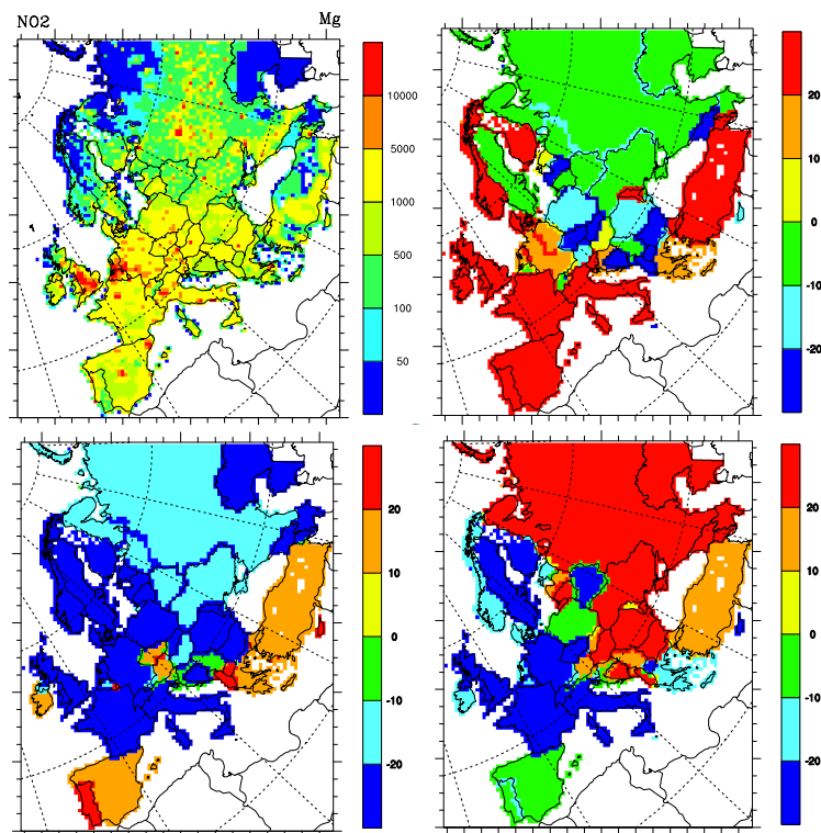
Fig. 5. Road transport emissions of NO 2 in 2005 (top left). Unit Mg. Difference in road transport emissions between 1980 and 1990 (top right), 1990 and 2000 (bottom left), 2000 and 2005 (bottom right). A negative number indicates a reduction. Unit: Percent.
