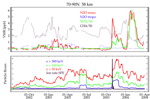
Fig. 8. As Fig. 7, but for 70–90° N.
