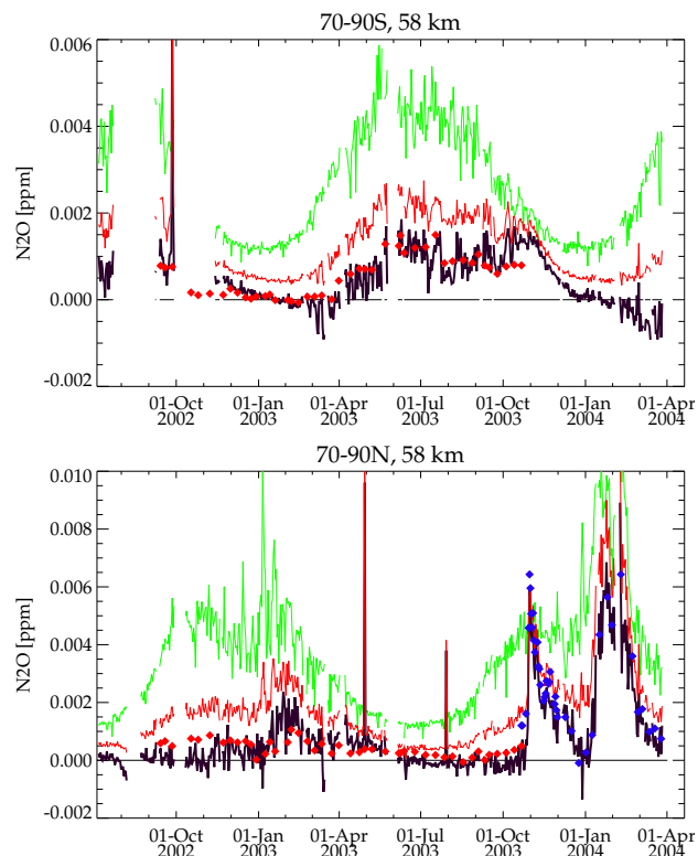
Fig. 5. 70–90° S (top) and 70–90° N (bottom) averages of ESA N 2 O vmr (reprocessed data version 4.61/4.62) with and without statistical correction (black and red solid lines, respectively), single measurement noise errors (green solid line), and N 2 O vmr retrieved at IMK/IAA (Versions V30_8.0 and V30_12.0 shown by red and blue diamonds, respectively) at 58 km. Spikes in the N 2 O averages on 26 September 2002 (SH), 29 April 2003 (NH), and 29 July 2003 (NH) are generated by spurious data.
