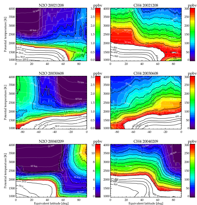
Fig. 1. Potential temperature-equivalent latitude daily mean cross sections of N 2 O (left) and CH 4 (right) vmr retrieved by IMK/IAA for the NH for 8 December 2002 (top), SH for 8 June 2003 (middle), and NH for 9 February 2004 (bottom). Data versions used are V3O_8.0 (top and middle) and V3O_12.0 (bottom). Mean geometric heights are indicated by dotted white lines. Note the different scale in the bottom left panel.
