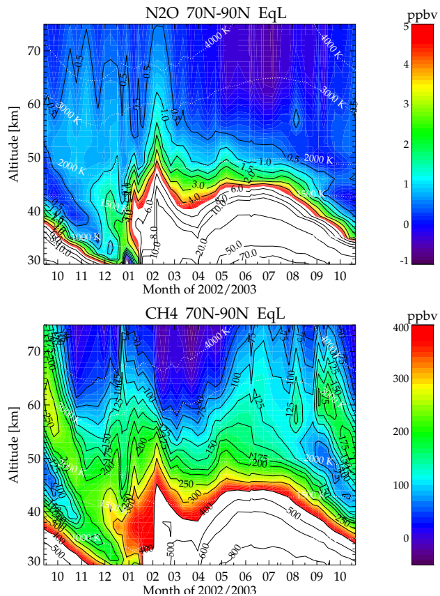
Fig. 3. As Fig. 2, but for equivalent latitudes 70–90° N.
