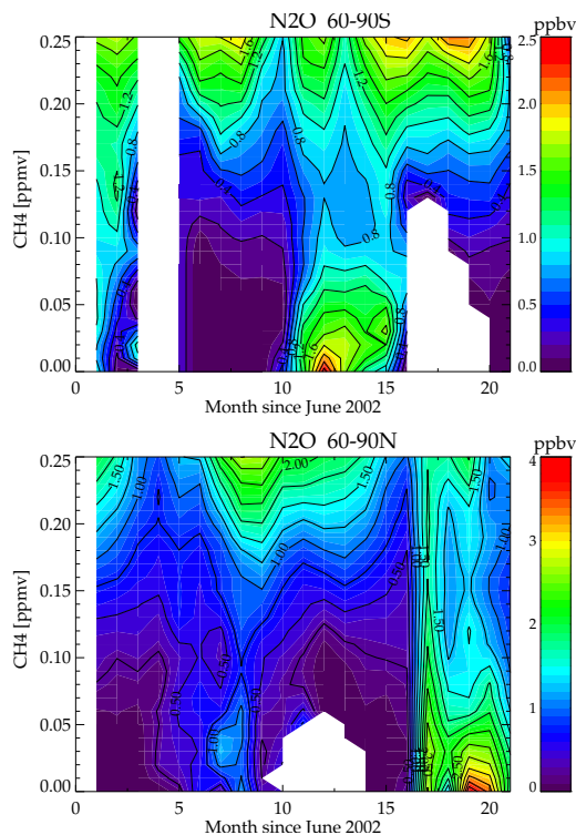
Fig. 6. Monthly mean median values of N 2 O PDFs at given CH 4 levels calculated from ESA 4.61/4.62 data products for 60–90° S (top) and 60–90° N (bottom). White regions reflect an availability of less than 30 observations at the corresponding CH 4 level. Note the different color scales for SH and NH!
