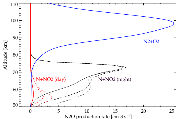
Fig. 10. Estimated EEP-related N 2 O productions by Reaction (R1) at polar night (solid black line) and day (SZA=80°) conditions (solid red line), as well as by Reaction (R2) (solid blue line) for the nominal scenario. Dashed and dotted lines represent N 2 O productions for the “high NO x ” scenario combined with the nominal and the “strong descent” temperature scenarios, respectively (only Reaction R1). See text for further details.
