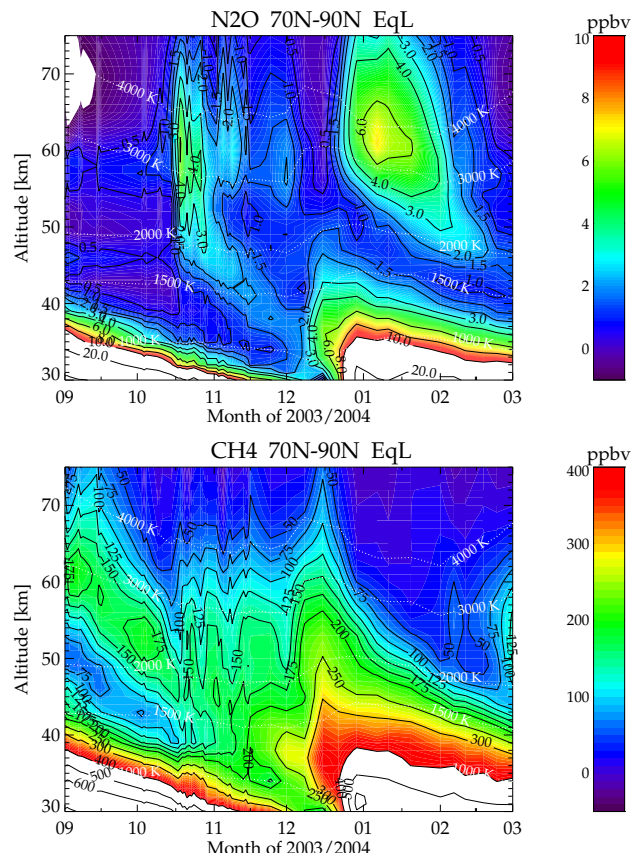
Fig. 4. Temporal evolution of N 2 O (top) and CH 4 (bottom) VMR retrieved by IMK/IAA (Version V3O_12.0) averaged over equivalent latitudes 70–90° N from September 2003 until March 2004. An area-weighting factor (cosine of equivalent latitude) has been applied. Mean potential temperatures are indicated by dotted white lines.
