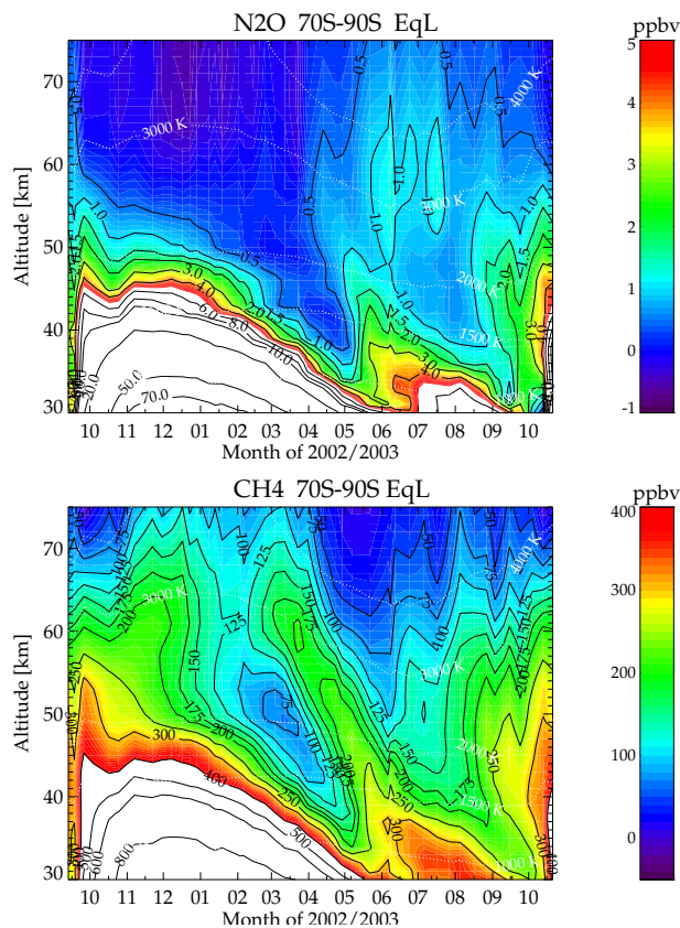
Fig. 2. Temporal evolution of N 2 O (top) and CH 4 (bottom) VMR retrieved by IMK/IAA (Version V3O_8.0) averaged over equivalent latitudes 70–90° S from September 2002 until October 2003. An area-weighting factor (cosine of equivalent latitude) has been applied. Mean potential temperatures are indicated by dotted white lines.
