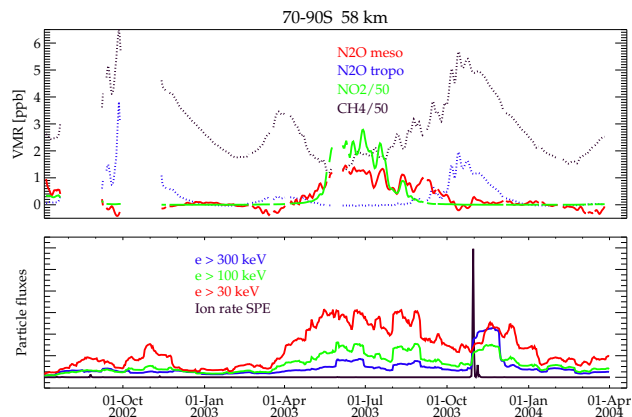
Fig. 7. Upper panel: Smoothed temporal evolution of the estimated mesospheric (solid red) and tropospheric (dotted blue) contributions to the observed N 2 O vmr, as well as NO 2 (solid green) and CH 4 (dotted black) vmrs (corrected ESA data) at 58 km averaged over 70–90° S. Note that NO 2 and CH 4 vmrs are scaled by a factor of 0.02. Lower panels: 30-day averages of integral precipitating electron fluxes within L>2.5 and 60–90° S with energies >30 keV (red), >100 keV (green), and >300 keV (blue) as measured by the MEPED instrument on NOAA. Atmospheric ionization rates at 0.3 hPa due to solar protons from Jackman et al. (2008) are also shown (black). Units are arbitrary.
