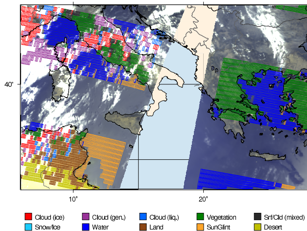
Fig. 1. Classification for the central Mediterranean Sea.
