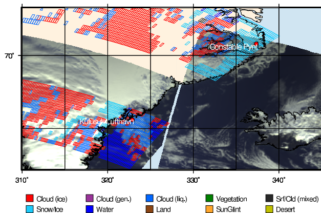
Fig. 3. Classification for Greenland for 16 Oct. 2007 (start time of the SCIAMACHY Orbit 29 423 was 14:10h UTC).
