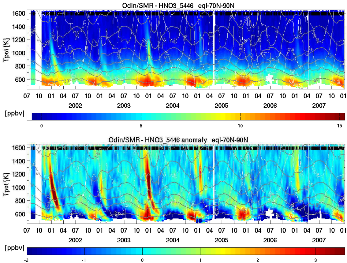
Fig. 3. Same as Fig. 2, but for Northern hemisphere high equivalent latitudes north of 70° N. Top: HNO 3 volume mixing ratio. Bottom: Absolute deviation from the mean profile.
