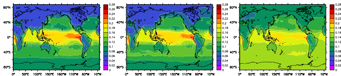
Fig. 11. Annual average \text{CHClBr}_2 (left), \text{CHCl}_2\text{Br} (middle) and \text{CH}_2\text{ClBr} (right) in the lowermost model layer in pmol/mol.
