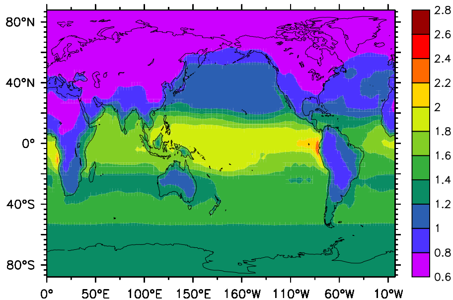
Fig. 5. Simulated annual average \text{CH}_2\text{Br}_2 in pmol/mol in the lowermost model layer.
