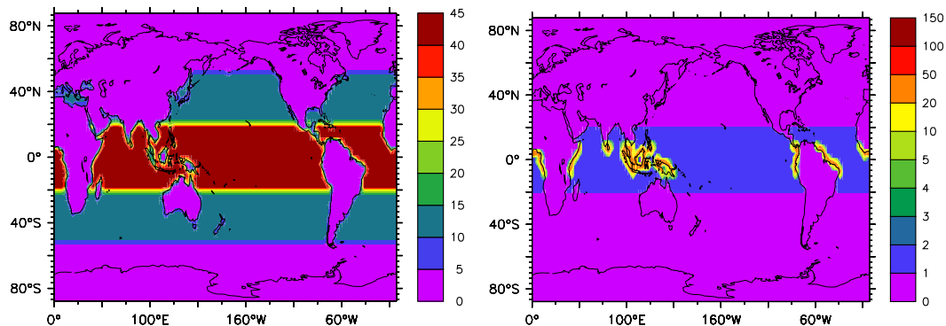
Fig. 1. Simulated annually integrated bromocarbon emission fluxes for \text{CH}_2\text{ClBr} (left \mu\text{g}/(\text{m}^2\text{yr}) ) and \text{CHBr}_3 (right, \text{mg}/(\text{m}^2\text{yr}) ).
