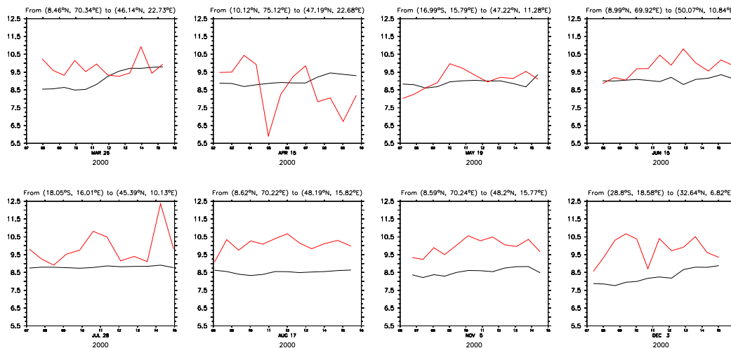
Fig. 22. Point to point comparison of \text{CH}_3\text{Br} mixing ratios from CARIBIC aircraft data (red line) and model results (black) as a function of time of day from March–December 2000.
