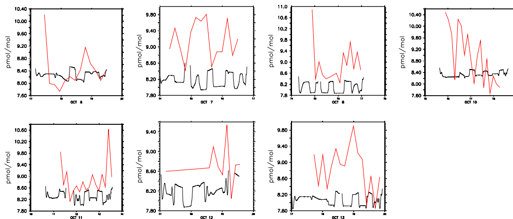
Fig. 23. Point to point comparison of \text{CH}_3\text{Br} mixing ratios from GABRIEL aircraft data (red line) and model results (black) as a function of time of day in October 2000.
