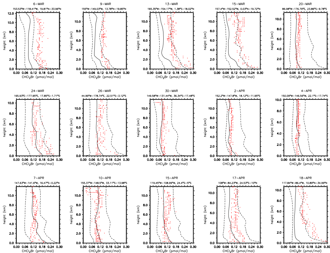
Fig. 15. As Fig. 4 but for \text{CHCl}_2\text{Br} and PEM-Tropics B.
