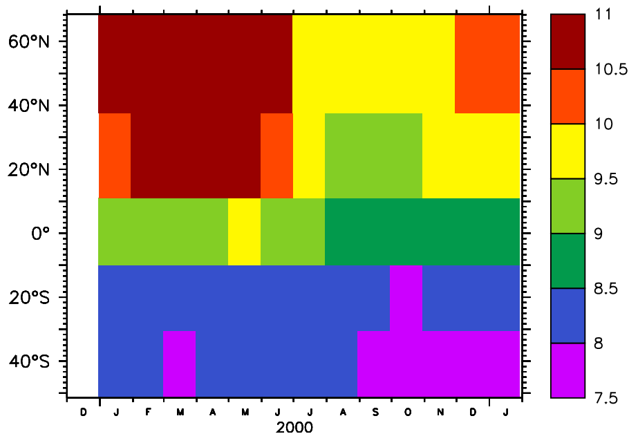
Fig. 2. Annual cycle of the surface \text{CH}_3\text{Br} mixing ratios (pmol/mol) as used by the submodel TNUDGE.
