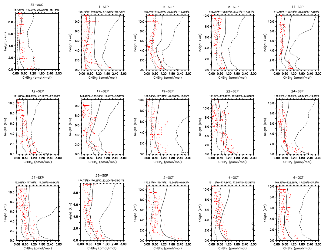
Fig. 4. \text{CHBr}_3 vertical profiles (pmol/mol) as measured during the PEM-Tropics-A DC8 campaign (red dots). The black lines show the simulated vertical profiles averaged over the flight period and area. The dashed lines indicate the simulated minimum and maximum \text{CHBr}_3 mixing ratios during the whole campaign period.
