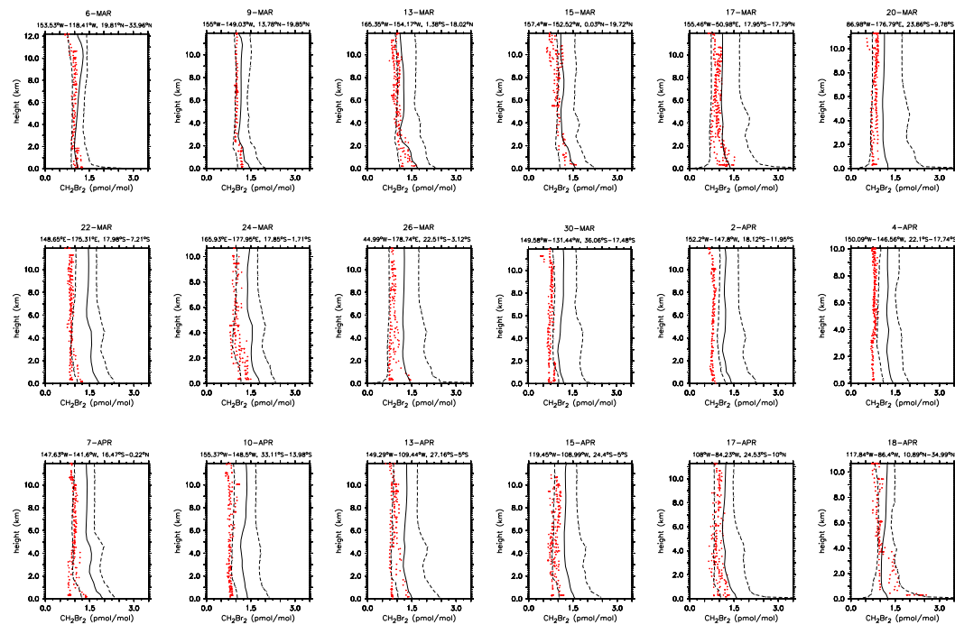
Fig. 6. As Fig. 4 but for \text{CH}_2\text{Br}_2 and the PEM-Tropics B campaign.
