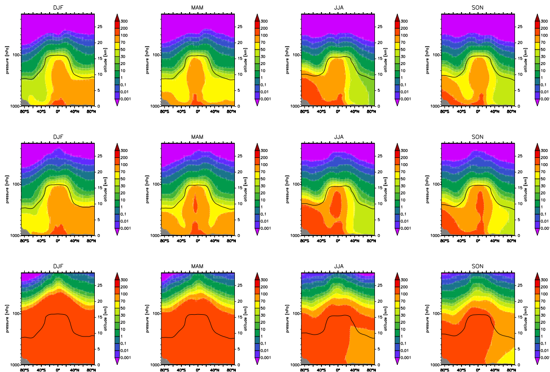
Fig. 12. Simulated vertical distribution of \text{CHClBr}_2 (upper row), \text{CHCl}_2\text{Br} (middle row) and \text{CH}_2\text{ClBr} (lower row) in fmol/mol. Shown are seasonal averages from left to right; DJF: December 1999–February 2000; MAM: March–May 2000; JJA: June–August 2000; SON: September–November 2000.
