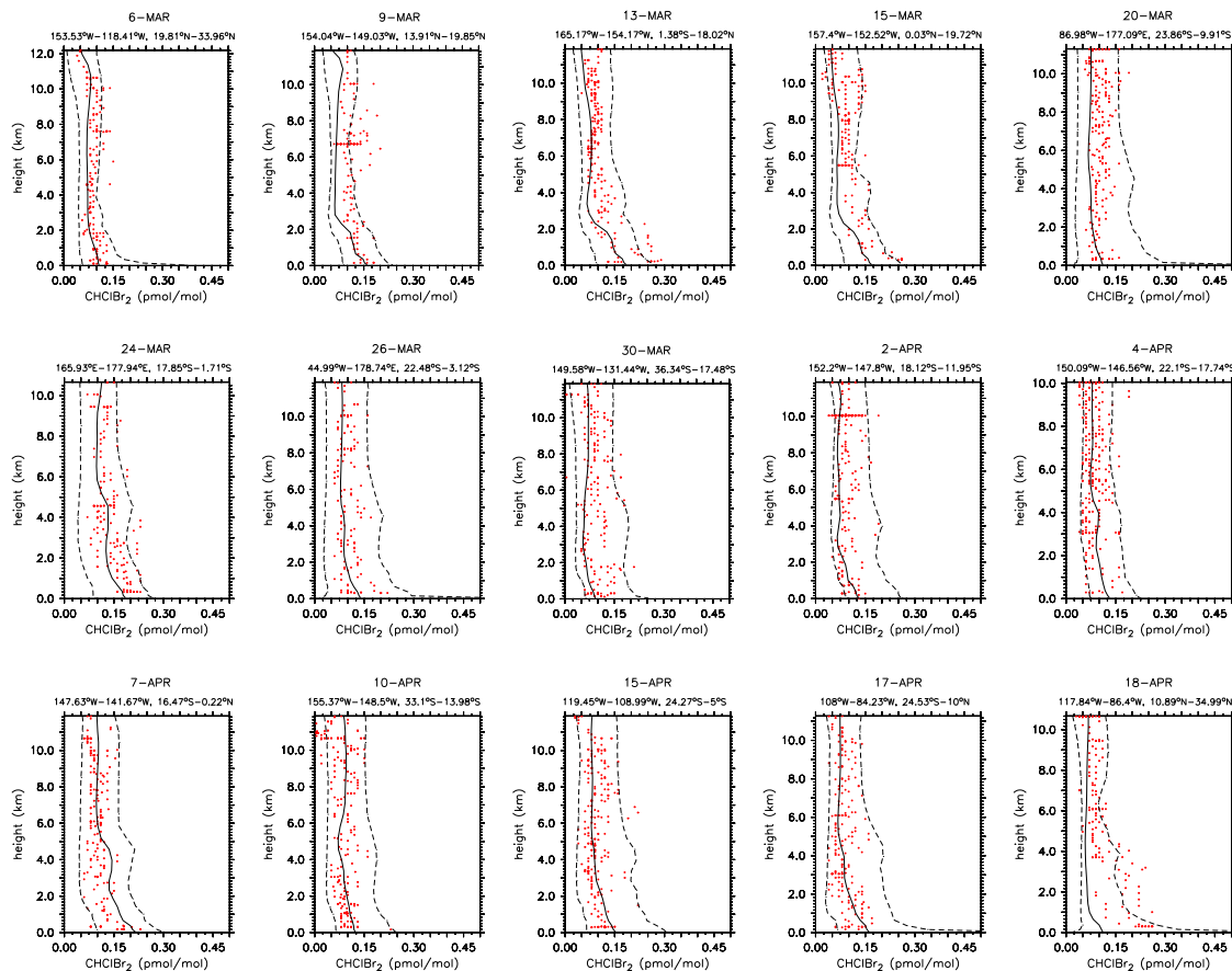
Fig. 13. As Figure 4 but for CHClBr 2 and the PEM-Tropics B campaign.
