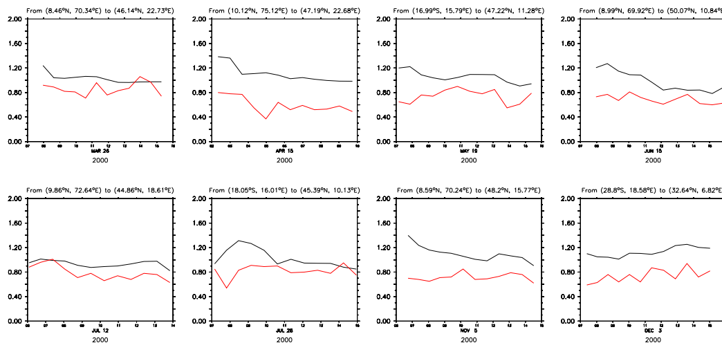
Fig. 7. Point to point comparison of \text{CH}_2\text{Br}_2 mixing ratios from the CARIBIC aircraft data (red line) and model results (black) as a function of time of day from March - December 2000.
