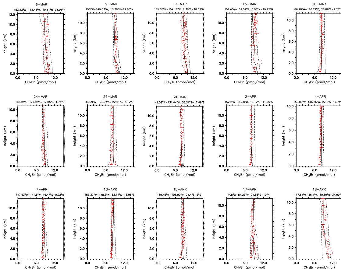
Fig. 20. \text{CH}_3\text{Br} vertical profiles (pmol/mol) as measured during the PEM-Tropics-B campaign (red dots). The black lines show the simulated vertical profiles averaged over the flight period and area. The dashed lines indicate the simulated minimum and maximum mixing ratios.
