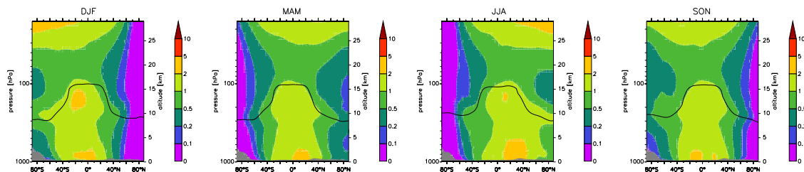
Fig. 10. Simulated vertical distribution of OH in 10^6/\text{cm}^3 . Seasons as in Fig. 9.
