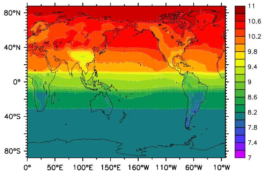
Fig. 17. (a) Annual average of \text{CH}_3\text{Br} (pmol/mol) in the lowest model layer.
