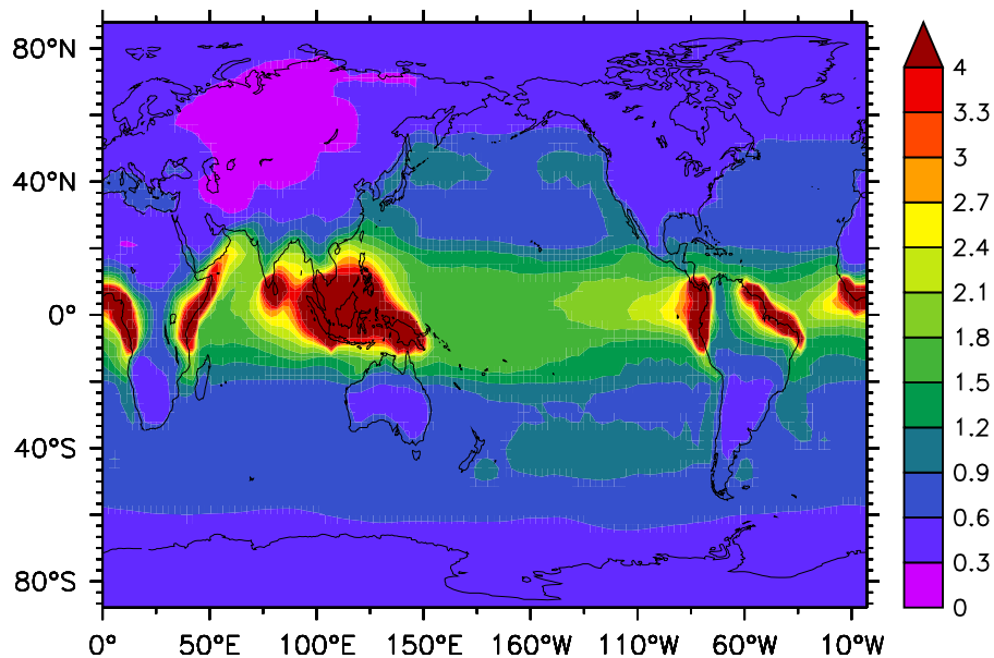
Fig. 3. Simulated annually averaged \text{CHBr}_3 mixing ratio (pmol/mol) in the lowermost model layer for the year 2000.
