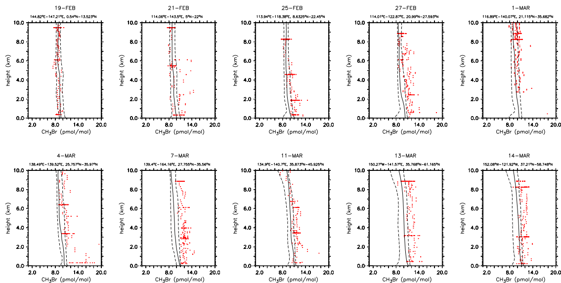
Fig. 21. As Fig. 4 for \text{CH}_3\text{Br} but from PEM-West B.
