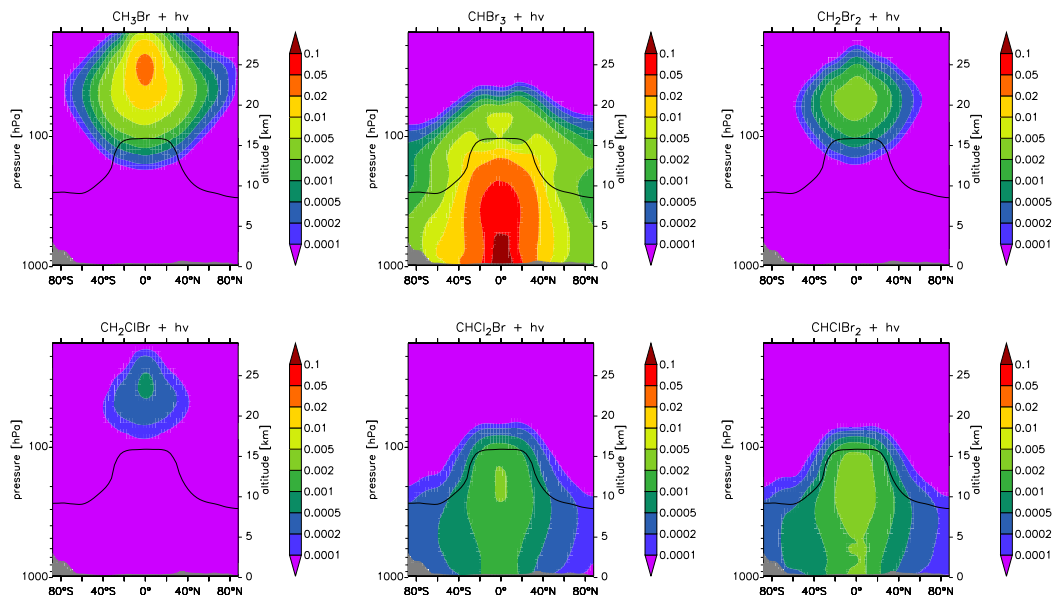
Fig. 24. Simulated production of Br radicals in g(Br)/s by photolysis of bromocarbons
