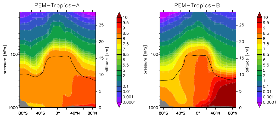
Fig. 19. Zonal averages of simulated \text{CH}_3\text{Br} mixing ratios (pmol/mol). The periods coincide with the PEM-Tropics A (5 August–6 October) and PEM-Tropics B (6 March–16 April) campaigns, though for the year 2000.
