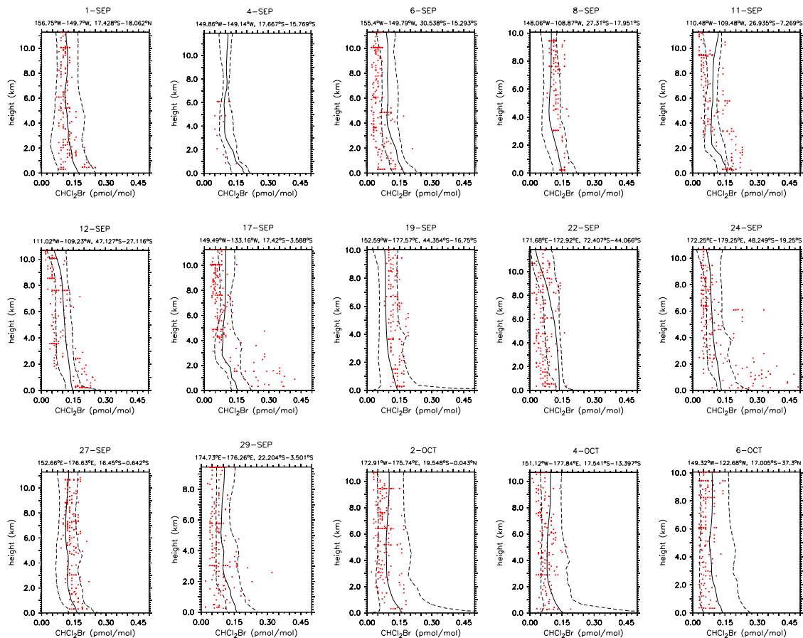
Fig. 14. As Fig. 4 but for \text{CHCl}_2\text{Br} .
