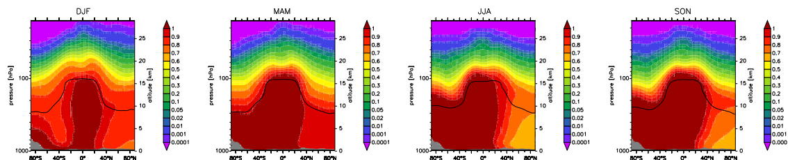
Fig. 9. Simulated vertical distribution of \text{CH}_2\text{Br}_2 in pmol/mol. Shown are seasonal averages; DJF: December 1999, January 2000, February 2000; MAM: March–May 2000; JJA: June–August 2000; SON: September–November 2000.
