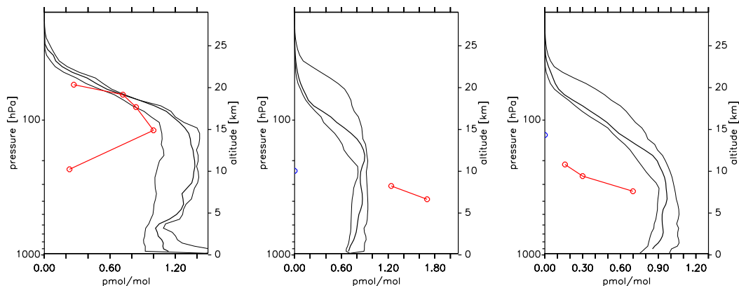
Fig. 8. \text{CH}_2\text{Br}_2 profiles in pmol/mol: Left: 9 April, Hyderabad, India; middle: 18 January, Kiruna, Sweden; right: 7 March, Kiruna, Sweden. The thick black line indicates the simulated profile. The thin black lines show the minimum and maximum simulated mixing ratios during a 14-day interval around the actual measurements. The red lines and the circles present the measurements of Kourtidis et al. (1996). The blue circles indicate measurements below the detection limit.
