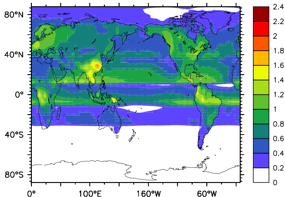
Fig. 18. Annual averages of the CH 3 Br pseudo-emission flux (10 11 molecules/(m 2 s)) resulting from the tracer nudging in the lowest model layer.
