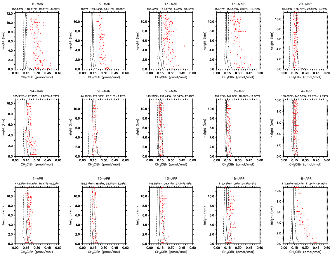
Fig. 16. As Fig. 4 but for \text{CH}_2\text{ClBr} and PEM-Tropics B.
