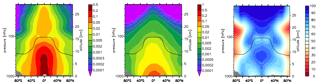
Fig. 25. Simulated zonally averaged Br radical production (in pmol/mol/day) by photolysis (left) and reaction with OH (middle) of bromocarbons, respectively. Here, photolysis of all six discussed bromocarbons and halons are taken into account. Right: Fraction (in%) of Br generated by photolysis to total Br production (photolysis+reaction with OH) from bromocarbons.
