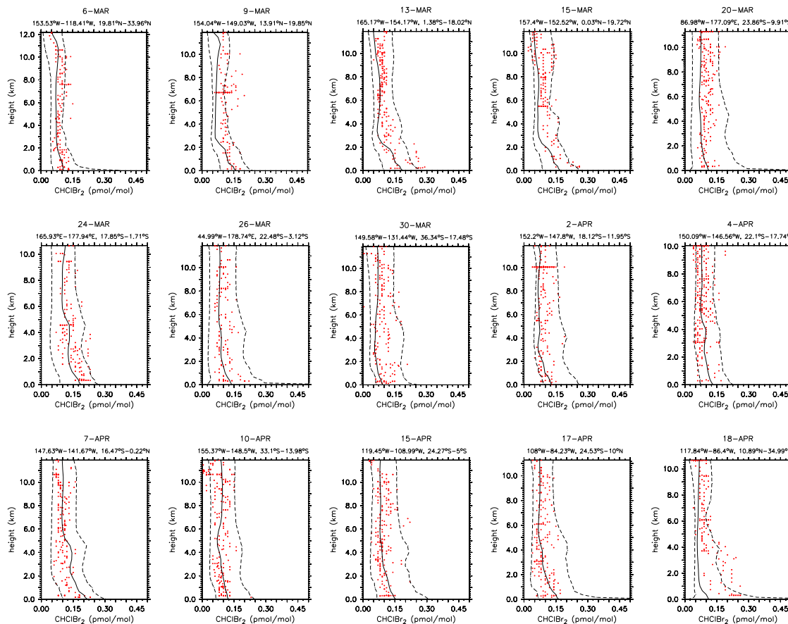
Fig. 13. As Figure 4 but for \text{CHClBr}_2 and the PEM-Tropics B campaign.
