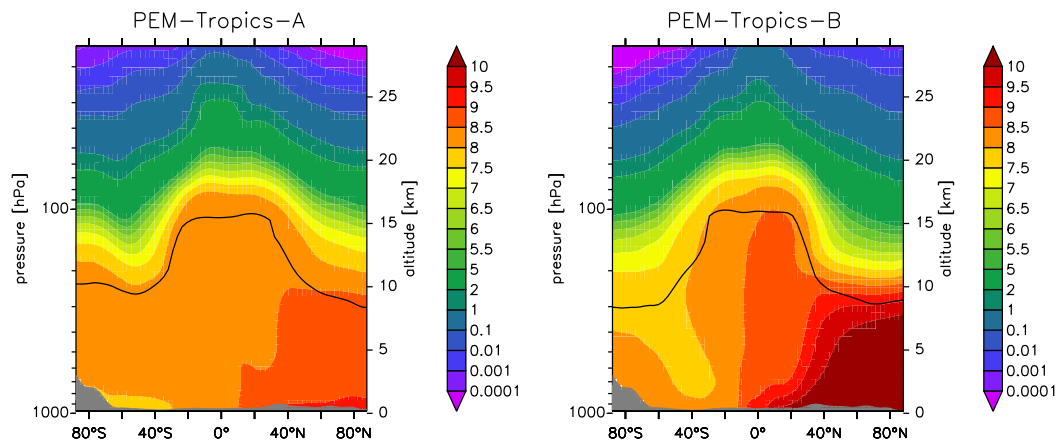
Fig. 19. Zonal averages of simulated \text{CH}_3\text{Br} mixing ratios (pmol/mol). The periods coincide with the PEM-Tropics A (5 August–6 October) and PEM-Tropics B (6 March–16 April) campaigns, though for the year 2000.
