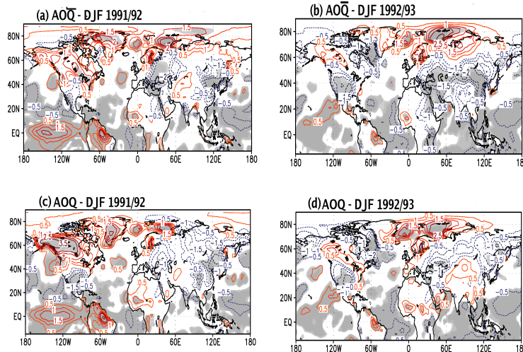
Fig. 6. 2 m temperature anomalies (K) for (a) AOQ: DJF 1991/1992 (b) AOQ: DJF 1992/1993, when the opposite QBO phase is prescribed; and for (c) AOQ: DJF 1991/1992 and (d) AOQ: DJF 1992/1993, when the observed QBO phase is prescribed. The shading denotes three levels (99%, 95% and 90%) of statistical significance in the order of lighter shading.
