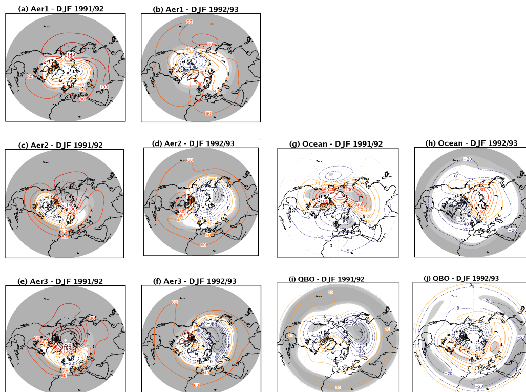
Fig. 4. Geopotential height anomalies at 30 hPa (m) for Aer1 ( a and b ); Aer2 ( c and d ); Aer3 ( e and f ); ocean response ( g and h ); qbo response ( i and j ); combined ocean and qbo (OQ) ( k and l ); combined aerosol and ocean (AO) ( m and n ); combined aerosol and QBO (AQ) ( o and p ); combined aerosol, ocean and QBO (AOQ) ( q and r ); for DJF 1991/1992 (left column) and DJF 1992/1993 (right column). Heavily shaded areas are significant at 99% level, lightly shaded at 90% significance level. Observed 30 hPa geopotential height response from ERA-40 (m) for DJF 1991/1992 ( s ) and DJF 1992/1993 ( t ).
