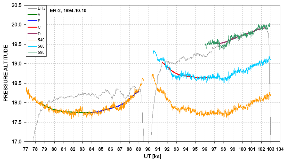
Fig. 2. Isentrop altitude cross-section for an ER-2 flight based in Christchurch, NZ. Altitudes for 540, 560 and 580 K isentrop surfaces are also represented by synoptic scale versions (smooth thick traces, flight segments A, B, C and D) using a 400 km double boxcar averaging procedure. The ER-2 flight altitude (light gray trace) shows a brief descent to ~15 km (made for in situ air sampling) at the south end of the flight (at ~90 ks).
