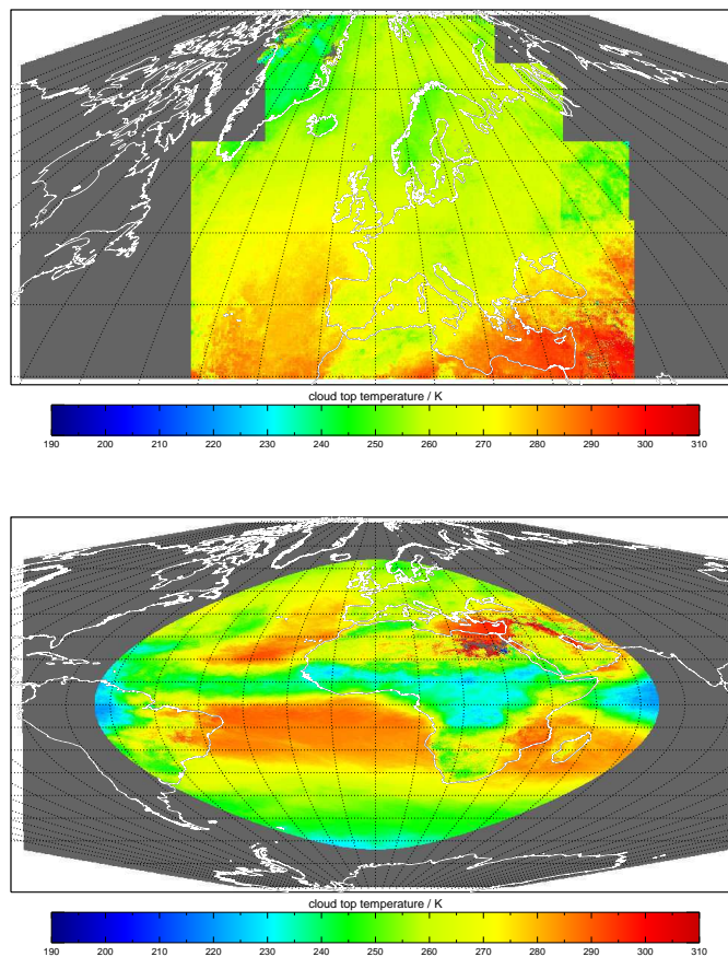
Fig. 1. Monthly mean cloud-top temperature for September 2007 derived from AVHRR observations (top panel) and from Meteosat9/SEVIRI (lower panel).
