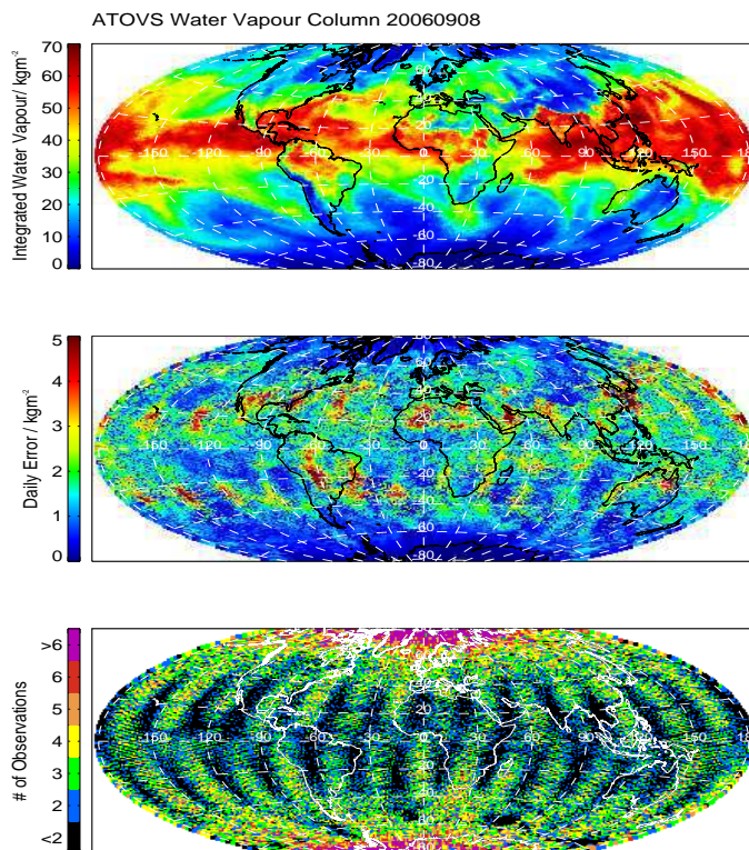
Fig. 4. Daily mean of vertically integrated water vapour (upper panel), daily error (middle panel) and number of independent observations (lower panel) derived from ATOVS data for 8 September 2006.
