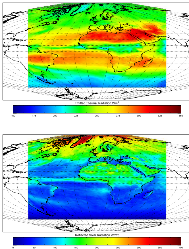
Fig. 6. Top of atmosphere monthly mean data for June 2007 of thermal emitted (top panel) and reflected solar flux (lower panel), respectively.
