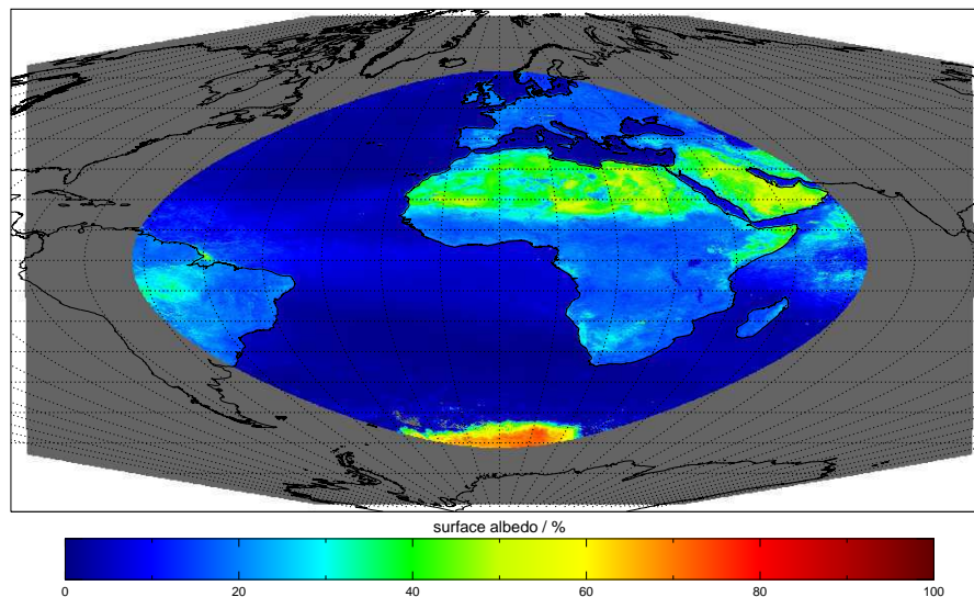
Fig. 8. Monthly mean surface albedo for September 2007 derived from Meteosat-9/SEVIRI observations.
