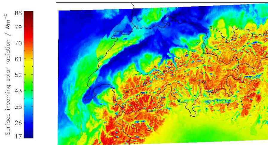
Fig. 10. Monthly mean surface incoming solar (SIS) radiation over complex terrain in Switzerland in December 2004 derived from Meteosat-8/SEVIRI and HRV observations. Here, slope and aspect from a high-resolution digital elevation model were used in the retrieval and SIS is clearly lower in east-west oriented Alpine valleys.
