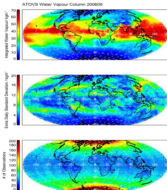
Fig. 3. Monthly mean vertically integrated water vapour (upper panel), corresponding extra daily standard deviation (middle panel) and number of independent observations (lower panel) derived from ATOVS data for September 2006.
