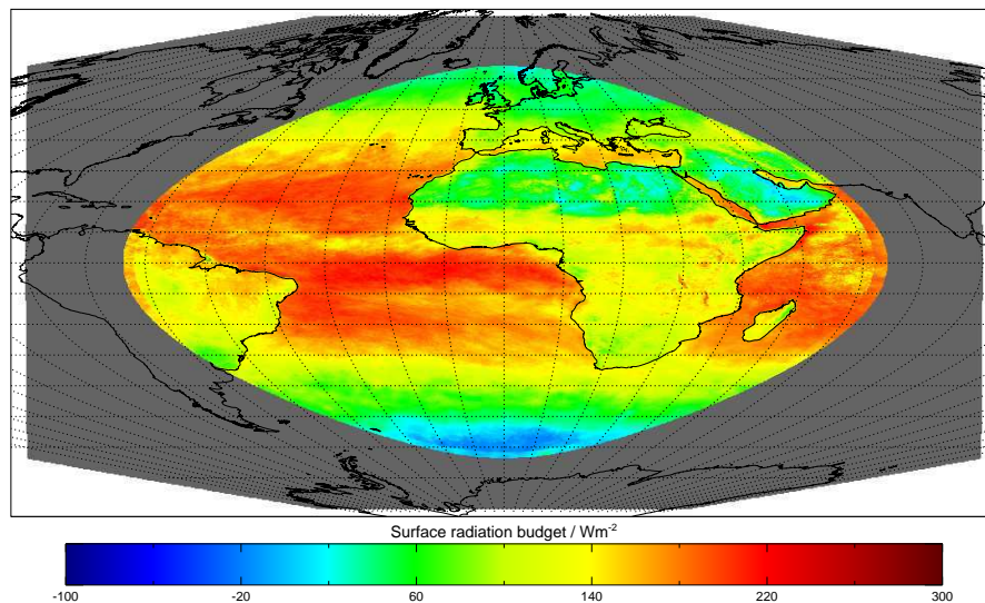
Fig. 9. Monthly mean surface radiation budget for September 2007 derived from Meteosat-9/SEVIRI observations.
