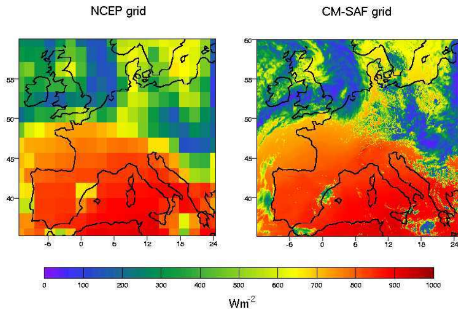
Fig. 7. Incoming solar radiation at surface level at NCEP (left panel) and CM-SAF (right panel) spatial resolution, respectively. Data from Meteosat-8/SEVIRI of 31 August 2006, 10:45 UTC.
