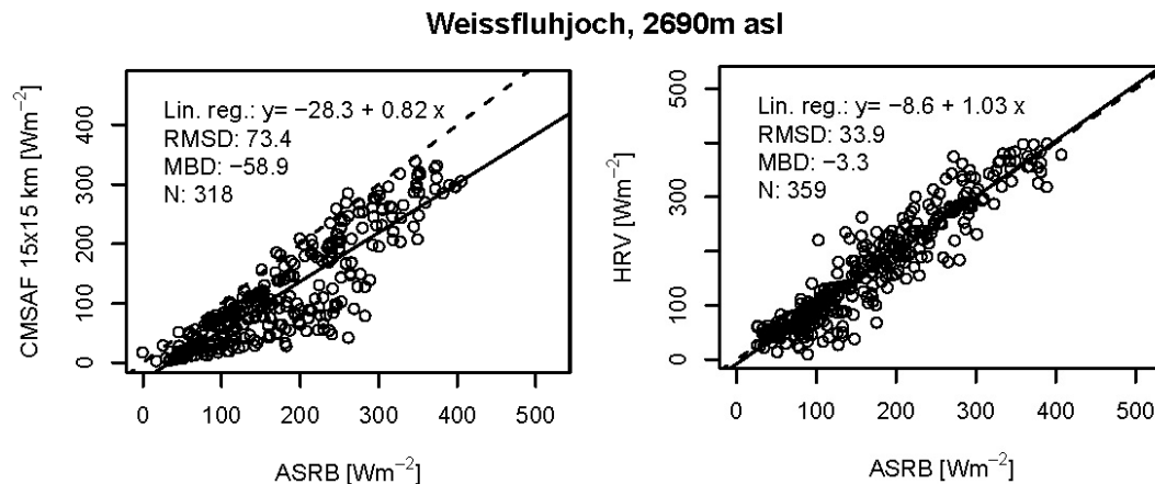
Fig. 11. Comparison of daily solar incoming radiation derived from SEVIRI solar channels (left panel) and the SEVIRI HRV channel (right panel) against ground-based measurements taken at Weissfluhjoch (Switzerland) for the period August 2004–July 2005.
