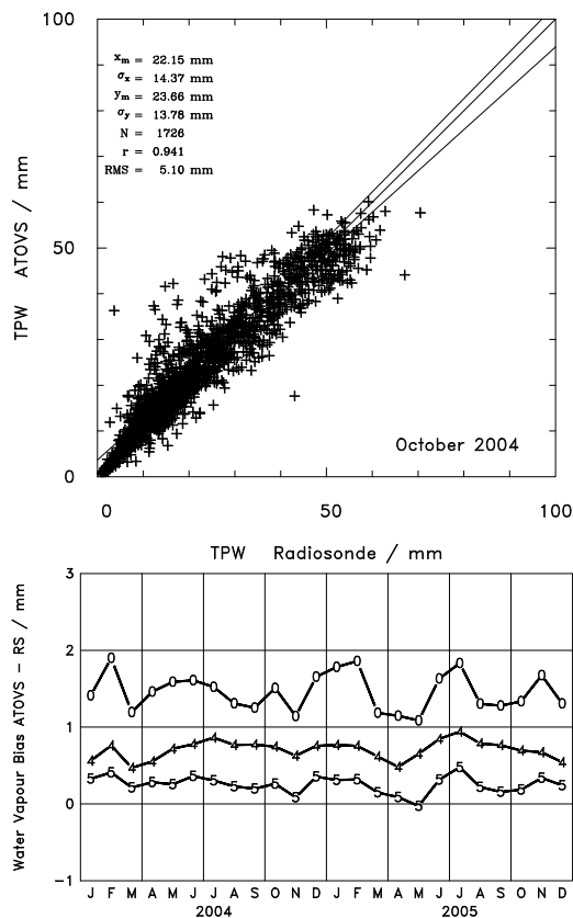
Fig. 5. Global comparison of daily averages of vertically integrated water vapour for October 2004 (top) and global mean bias error for the total column (curve denoted by 0) and the layers 1000–850 (denoted by 5) and 850–700 hPa (denoted by 4) (bottom).
