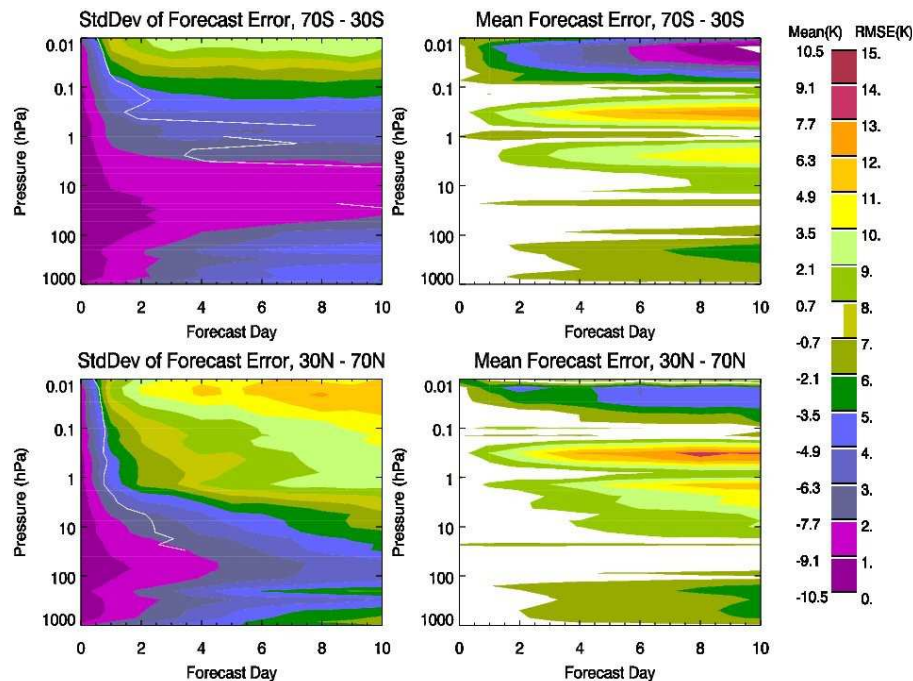
Fig. 9. Forecast mean error and error standard deviation relative to the analysis at 30^{\circ} – 70^{\circ} S (top row) and 30^{\circ} – 70^{\circ} N (bottom row). Results are an average of 12 10-day forecasts. White line marks the forecast day at which the error standard deviation increases above the estimated accuracy of the assimilation (based on MLS and SABER O-F statistics above 30 hPa, see text for details).
