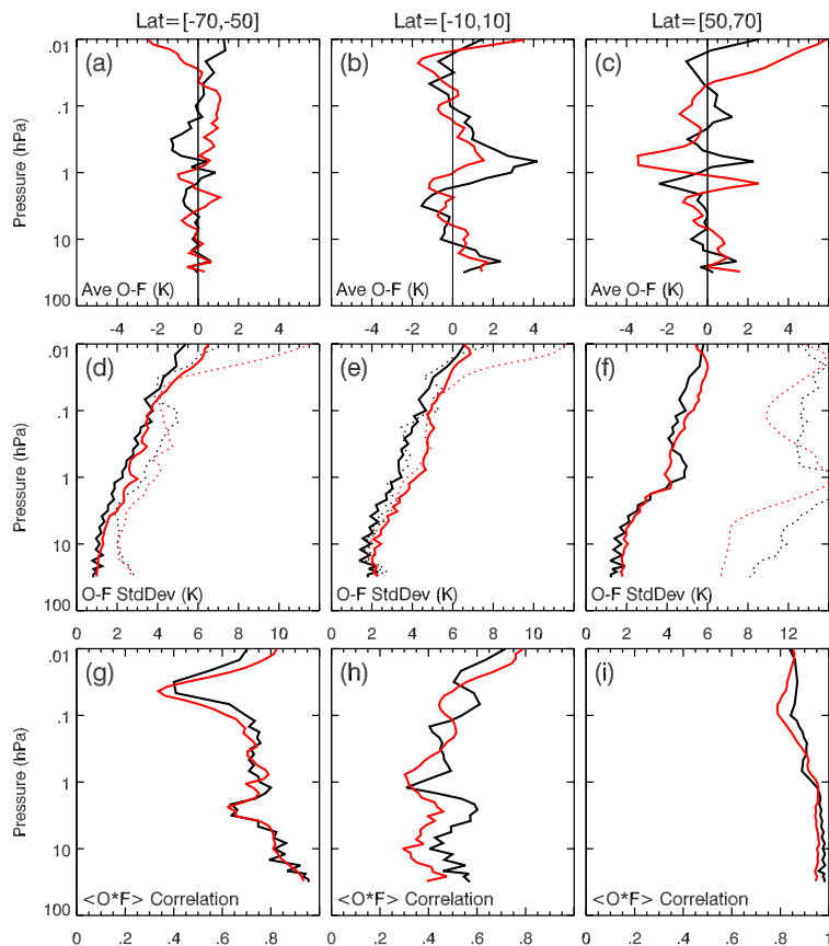
Fig. 7. O-F statistics for the January–February 2006 analysis period: black=MLS, red=SABER in three latitude bands of 50°–70° S (left), \pm 10^\circ (center) and 50°–70° N (right), (a–c) Global average O-F; (d–f) O-F standard deviation; (g–i) Correlation coefficient between observations and forecast. Dotted curves in (d–f) plot corresponding O standard deviations only.
