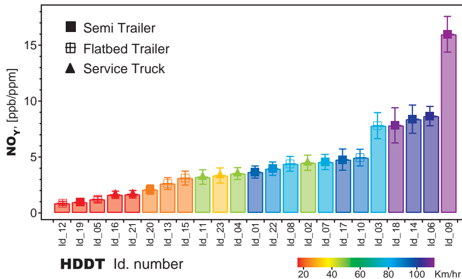
Fig. 6. NO_y/CO_2 on-road emissions of individual HDDTs measured in Austin TX, by vehicle speed.
