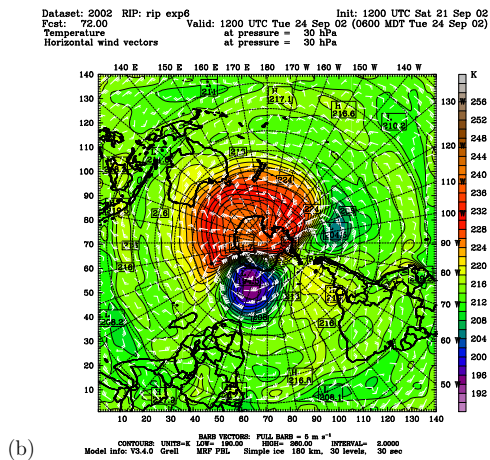
Fig. 2. Temperature and winds on the 30 hPa surface at 12:00 UTC on 24 September 2002 from (a) an analysis and (b) a 72-h forecast simulation.
