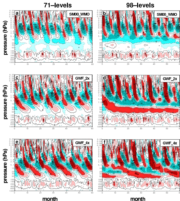
Fig. 6. Time-height evolution of zonal-mean zonal wind at the equator for two sets of 5y present-day simulations based on the SM00_WMO configuration of DYN-MAM. Simulations employing the standard 71-level version of CMAM are on the left while simulations employing a 98-level version of the model with enhanced vertical resolution in the stratosphere are on the right. From top to bottom, the flux of non-orographic gravity waves is constant at all latitudes (panels a and b ), increased in the tropics by a factor of 2 (panels c and d ), and by a factor of 4 (panels e and f ).
