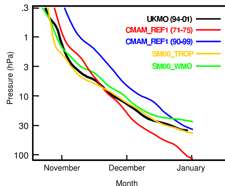
Fig. 5. Time evolution of the zero line of the zonal-mean wind at 60° S based on the climatological mean annual cycle. The observed evolution as represented by UKMO reanalysis data (Swinbank and O'Neill, 1994) is shown in black.
