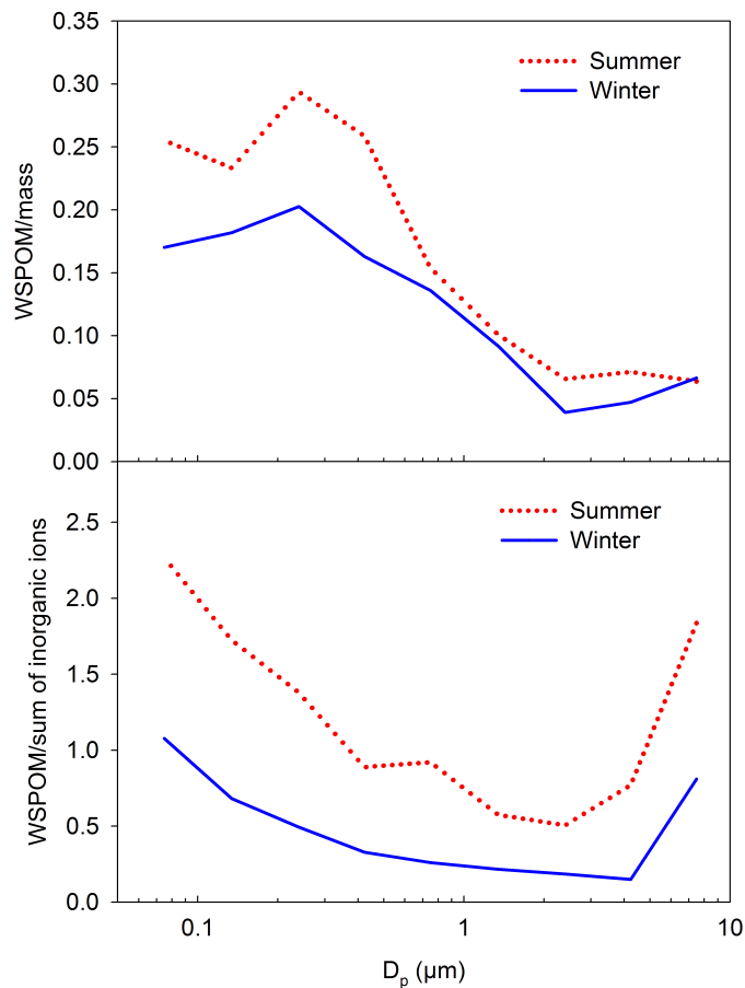
Fig. 7. The calculated WSPOM/mass-ratio and WSPOM/inorganic ions ratio for aerosols originating from clean arctic areas in summer and in winter.
