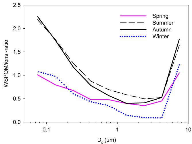
Fig. 3. The WSPOM/inorganic ions-ratio in different size classes in MOUDI collections for each season: spring (Mar–May), summer (Jun–Aug), autumn (Sep–Nov), and winter (Dec–Feb).
