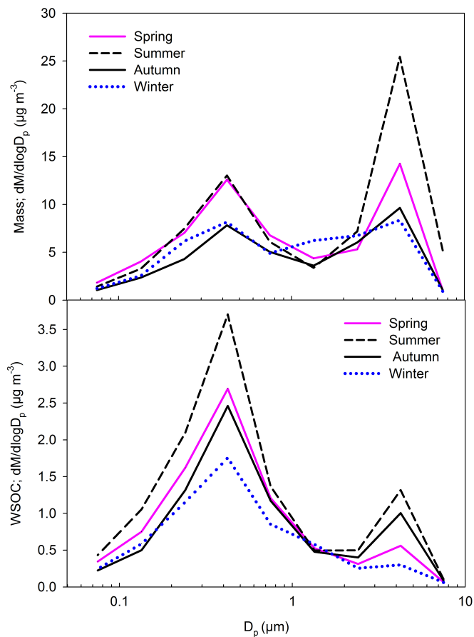
Fig. 2. The mass and WSOC size distributions for each season: spring (Mar–May), summer (Jun–Aug), autumn (Sep–Nov), and winter (Dec–Feb).
