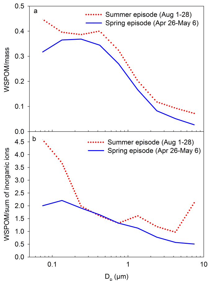
Fig. 6. The calculated WSPOM/mass-ratio (a) and WSPOM/inorganic ions ratio (b) for biomass burning aerosols originating from the wild land fire areas in spring (26 Apr– 6 May 2006) and in summer (1–28 Aug 2006).
