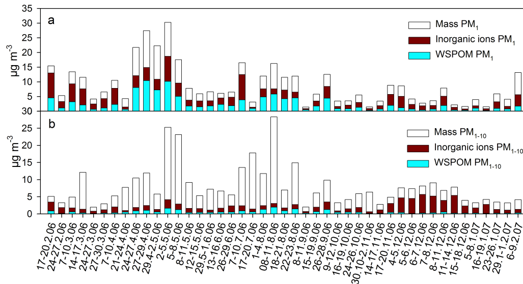
Fig. 1. Concentrations of mass, inorganic ions and WSPOM ( \mu\text{g m}^{-3} ) in \text{PM}_1 (a) and \text{PM}_{1-10} (b) in the MOUDI collections between February 2006 and February 2007.
