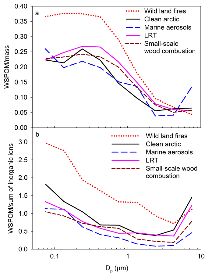
Fig. 5. The WSPOM/mass -ratio (a) and WSPOM/inorganic ions -ratio (b) for collections representing the five different aerosol sources; LRT, clean arctic, wild land fires, marine and small-scale wood combustion.
