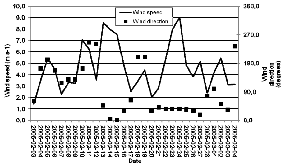
Fig. 1. The average wind speed ( \text{m s}^{-1} ) and wind direction (degrees) for the measurement period of this study. The averages are calculated from noon each day and the day indicated in the figure is the same date as when the filters were collected. 0 (and 360) degrees is wind coming from north, 90 degrees is east, 180 degrees south and 270 degrees is westerly winds.
