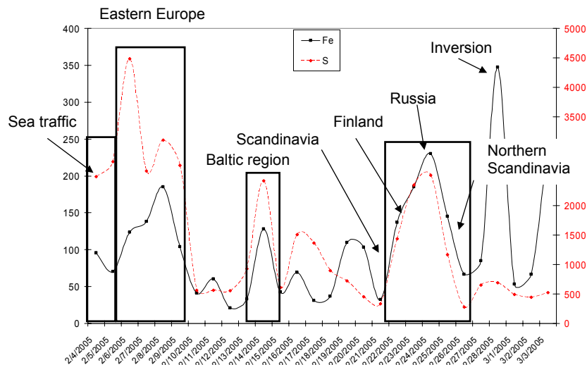
Fig. 3. The S and Fe concentration at the Femman measurement site given on a daily basis together with indications of the possible origin of the air masses. The inversion period between 27 and 28 February is indicated in the figure.
