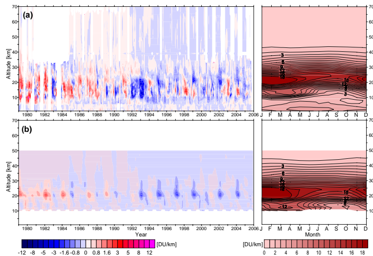
Fig. 6. (a) Ozone anomalies (left) and mean annual cycle (right) for data extracted from the BDBP, for altitudes between 1 km and 70 km and for the latitude zone from 40° N to 50° N. (b) same as a), for data extracted from R&W. White areas indicate where no values are available.
