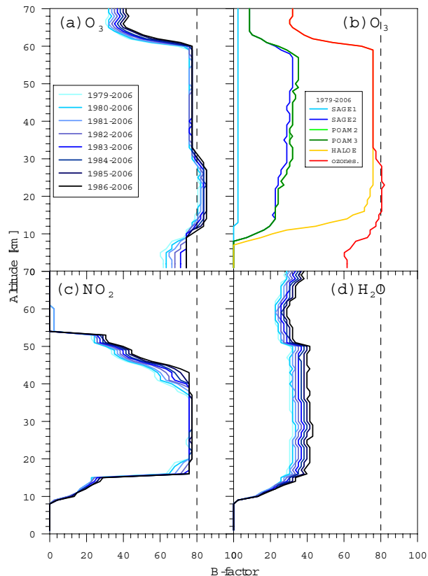
Fig. 4. B-factors for O 3 , NO 2 and H 2 O as a function of changing time period (panels (a) , (c) and (d) respectively) and for O 3 as a function of changing data source (panel (b) ). The 80% level in all panels is shown for reference.
