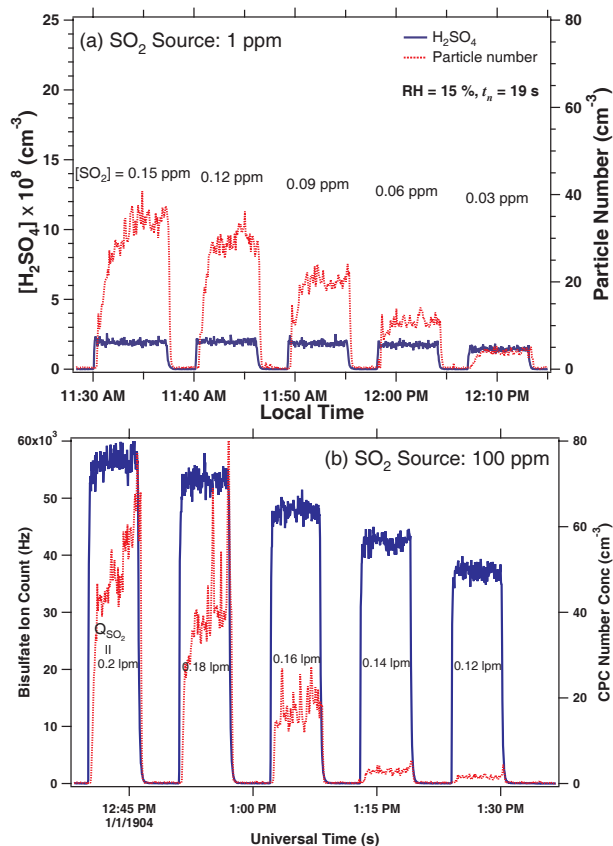
Fig. 5. The measured particle number concentrations as a function of the residual [H 2 SO 4 ] with the 1 ppm (a) and 100 ppm (b) SO 2 source cylinder at 288 K. The initial [SO 2 ] are shown in ppm in the figures.
