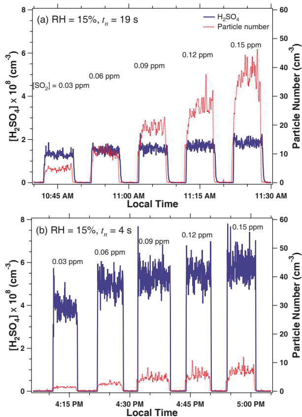
Fig. 6. The measured particle number concentrations as a function of the residual [\text{H}_2\text{SO}_4] with (a) nucleation time t_n = 19 s and (b) t_n = 4 s at 288 K. The initial [\text{SO}_2] are shown in ppm in the figures.
