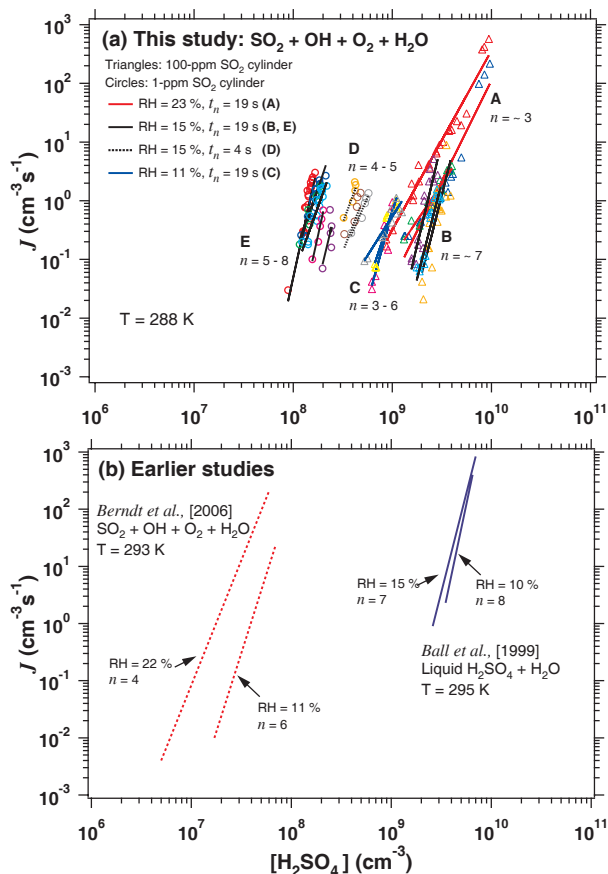
Fig. 14. The measured nucleation rates J as a function of [\text{H}_2\text{SO}_4] for (a) the present \text{SO}_2 + \text{OH} experiments and (b) from earlier studies. The linear lines are the results of power regression on the experimental data. The calculated wall loss factors (WLFs) corresponding to our experimental conditions are shown in Fig. 3. In Ball et al. (1999), \text{WLF}=22 . Berndt et al. (2006) did not provide WLFs.
