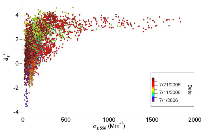
Fig. 14. Second derivative ( \ddot{a}'_s ) versus scattering coefficient ( \sigma_{s,550} ) for the whole campaign, including 23–25 July.
