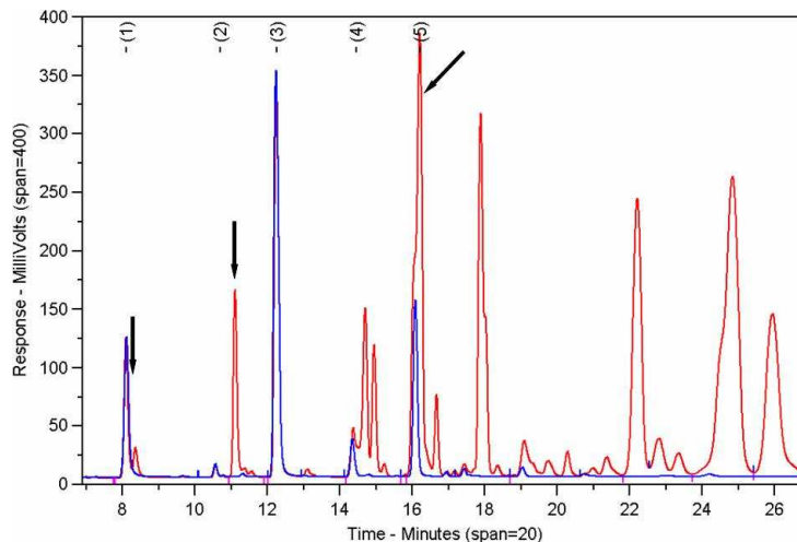
Fig. 1. Comparison of the chromatograms from two air samples taken at the Taunus Observatory operated by the University of Frankfurt. Trace gases were concentrated cryogenically from 1 l of air and detected using an ECD. The blue line represents “normal” air while the red line is the plume sample taken on the 2 October 2007 which showed a number of unidentified large signals. The known large peaks are \text{CF}_2\text{Cl}_2 [CFC-12, (1)], \text{CF}_2\text{ClBr}/\text{CF}_2\text{ClCF}_2\text{Cl} [Halon-1211/CFC-114, coeluting, (2)], \text{CFCl}_3 [CFC-11, (3)], \text{CF}_2\text{ClCFCl}_2 [CFC-113, (4)] and \text{CCl}_4 (5). Three of the unknown substances could be identified by now and are labelled with black arrows: trifluorochloroethene at 8.4 min, 3-chloropentafluoropropene at 11.1 min and 4,4-dichlorohexafluoro-1-butene at 16.2 min.
