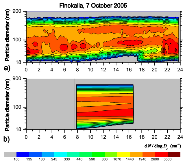
Fig. 9. Particle number size distributions at Finokalia on 7 October 2005: (a) Measurement illustrating the gradual disappearance of Aitken mode particles, (b) box model simulation starting at 08:00 LT and involving only condensation and particle coagulation.
