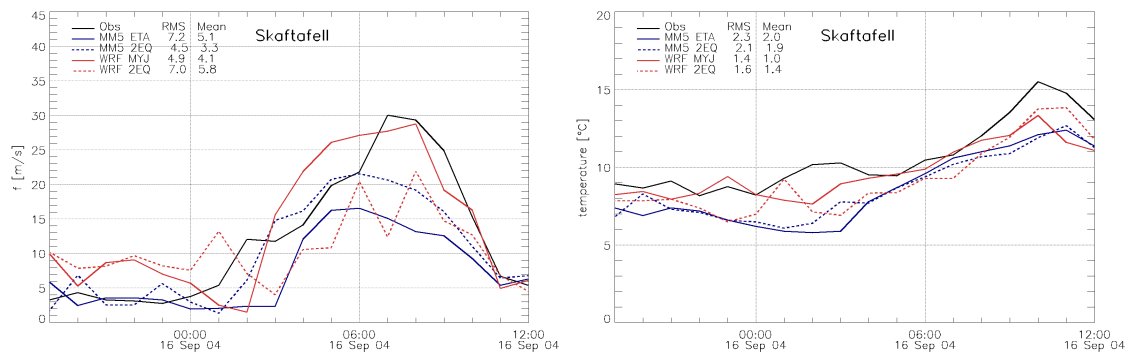
Fig. 4. Observed (solid black) and simulated (solid blue – MM5/ETA, blue dash – MM5/2EQ, solid red – WRF/MYJ, red dash – WRF/2EQ) 10 m wind speed ( m s^{-1} ) (left) and 2-m temperature ( ^{\circ}C ) (right) at station Skaftafell (WMO# 4172 – SKAFT) in the lee of Mnt. Öræfajökull.
