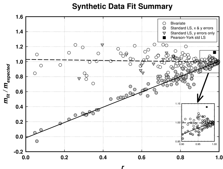
Fig. 3. Ratio of fitted to expected slopes ( m_{\text{fit}}/m_{\text{expected}} ) from standard least-squares and the Williamson-York bivariate method versus r -values from Eq. (3). Errors in both the x and y variables lead to systematic errors the slope from standard least squares. Slopes from the bivariate method show no such systematic variation with r .
