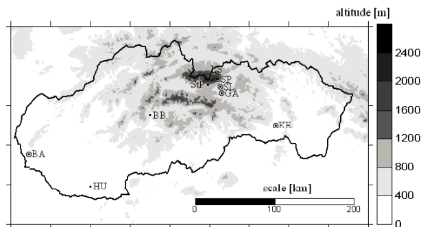
Fig. 1. Investigated territory with surface altitude and border of Slovakia. The places with measurements of total solar radiation are designed by black dots, places with UV radiation measurements are labelled by rings. The abbreviations of observatories relate to Table 1.
