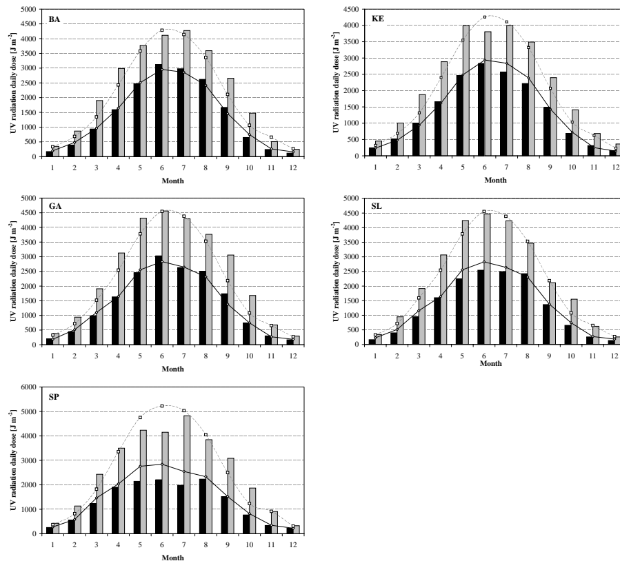
Fig. 4. Monthly mean values of the erythemal UV radiation calculated from measured data at stations equipped by the UV-radiometers (abbreviations in Table 1) for the 2002–2004 period (black columns), the modelled clear-sky erythemal UV radiation (grey squares) and the erythemal UV radiation attenuated by mean cloudiness (white diamonds). The erythemal UV radiation was modelled for average total ozone and typical snow conditions (the surface covered by snow was assumed from altitudes with snow incidence probability of 50%).
