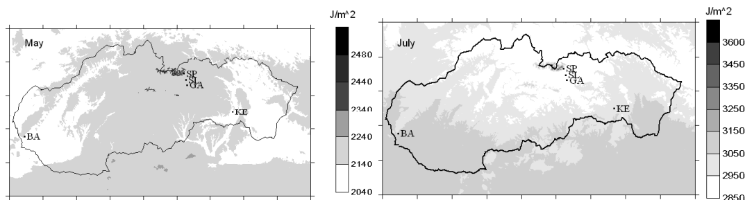
Fig. 3. Modelled erythemal UV-radiation daily doses for May and for July assuming mean attenuation by clouds. The UV radiation daily doses were calculated for the first day of month and corresponded monthly average values of the total ozone, the cmf_{UV} and appropriate snow conditions (the surface covered by snow was assumed from altitudes with snow incidence probability of 50%).
