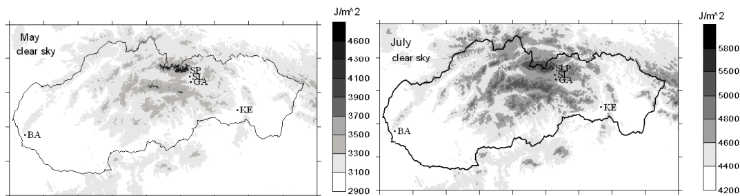
Fig. 2. Modelled clear-sky erythemal UV-radiation daily doses for May and for July. The clear-sky UV radiation daily doses were calculated for the first day of month and corresponding monthly average values of the total ozone and appropriate snow conditions (the surface covered by snow was assumed from altitudes with snow incidence probability of 50%).
