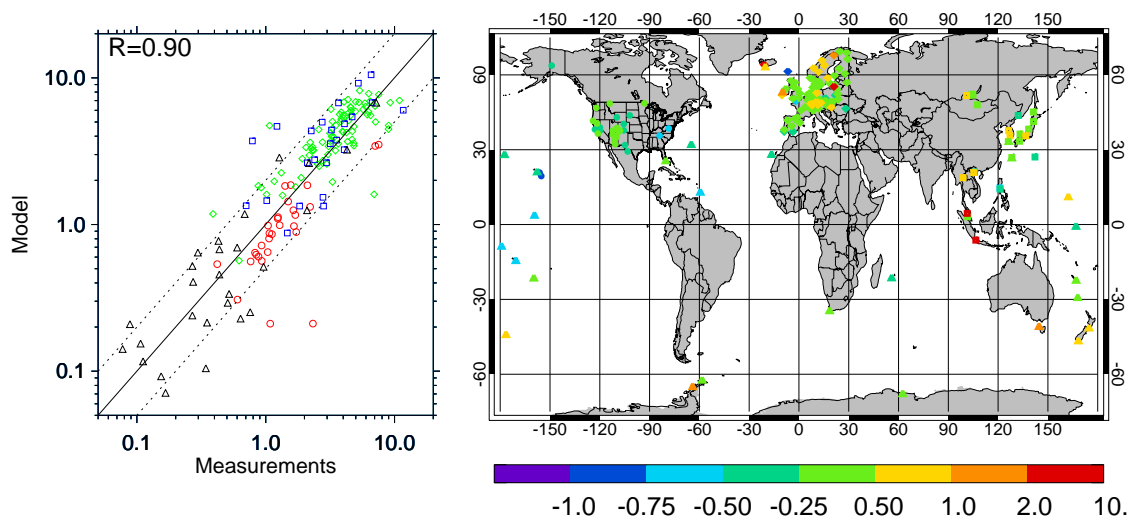
Fig. 2. Scatter plot (left panel) and the relative difference (i.e., (\text{model} - \text{obs}) / \text{obs} , right panel) between the simulated (MOZART2, early 1990s) and observed annual mean sulfate concentrations ( \text{SO}_4^{2-} ; unit: \mu\text{g}\cdot\text{m}^{-3} ). Observations are from RSMAS (1980s–1990s average, University of Miami, triangles), IMPROVE (1990–1992 average, circles), EMEP (1990–2002 average, diamonds), and EANET (2000–2004 average, squares).
