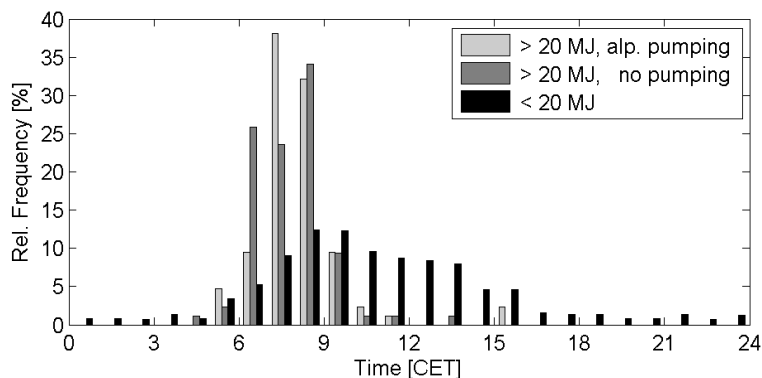
Fig. 9. Diurnal variation of relative frequency of O_3 events for days with high irradiation and Alpine Pumping (light grey, N=84 ), with high irradiation but without Alpine Pumping (dark grey, N=85 ) and for days with total irradiated energy of less than 20 \text{ MJ m}^{-2} (black, N=587 ).
