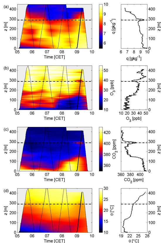
Fig. 7. Time-height cross sections and profiles of (a) specific humidity q , (b) \text{O}_3 mixing ratio, (c) \text{CO}_2 mixing ratio, and (d) potential temperature \theta for the morning of 5 September 2005. The actual flight path of the tethered balloon is indicated by the thin black line. Profiles on the right side show the upward scan of the tethered balloon at the time when the \text{O}_3 drop reached the TOP station (corresponding to the actual flight path marked with a thick black line).
