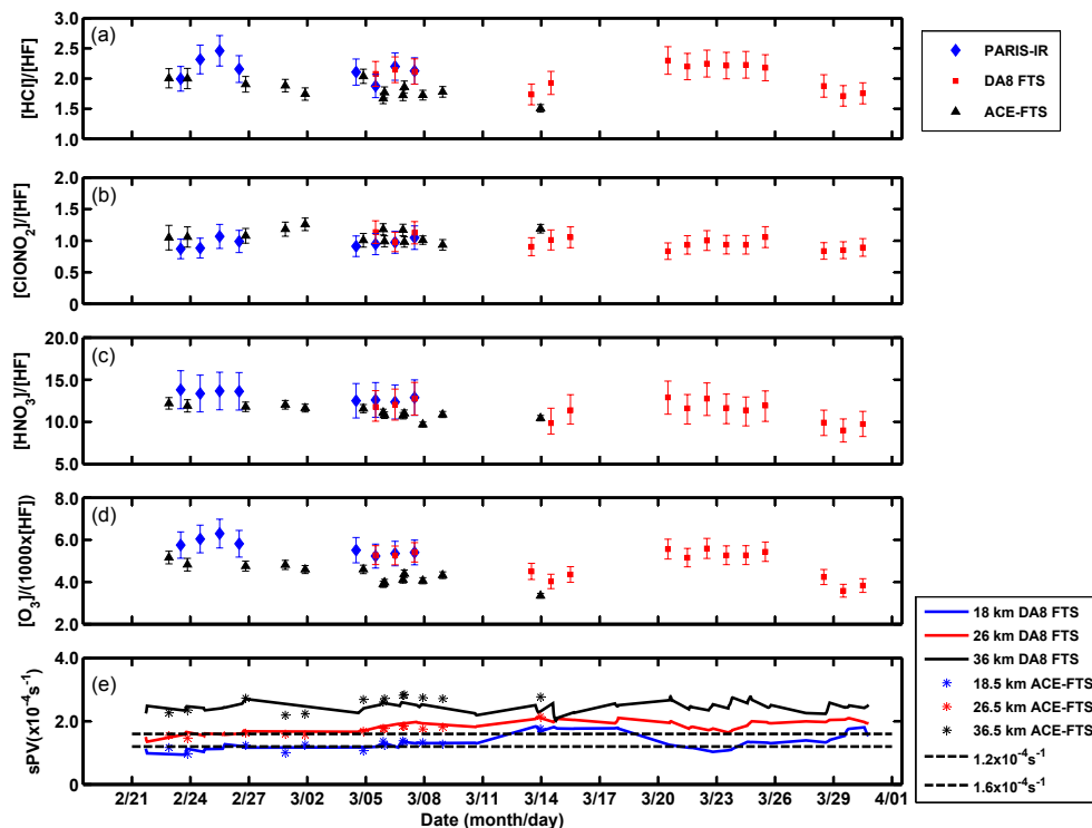
Fig. 7. Time evolution of total column density ratio for HCl (a), \text{ClONO}_2 (b), \text{HNO}_3 (c), and \text{O}_3 (d), normalized by HF from the observations using PARIS-IR (blue diamonds) and the DA8 FTS (red squares) during the 2006 Canadian Arctic ACE Validation Campaign. The partial column density ratios calculated from the ACE-FTS results are also shown (black triangles). The altitude ranges of the partial column density ratios of [\text{HCl}]/[\text{HF}] , [\text{ClONO}_2]/[\text{HF}] , [\text{HNO}_3]/[\text{HF}] , and [\text{O}_3]/[\text{HF}] from ACE-FTS are 13.5–44.5 km, 14.5–30.5 km, 13.5–31.5 km and 13.5–44.5 km, respectively. The altitude range of the total column density ratios from the DA8 FTS and PARIS-IR is surface – 100 km. (e) The scaled potential vorticity (sPV) at altitudes of 18 km, 26 km, and 36 km along the optical paths of the DA8 FTS measurements and those of ACE-FTS from GEOS-4 analyses. The dashed lines indicate 1.2 and 1.6 \times 10^{-4} \text{ s}^{-1} , the edges of the polar vortex. Error bars for the ratios are calculated by propagating the error in the total column densities given in Table 2 for the DA8 FTS and PARIS-IR, and the spectral fitting error for the ACE-FTS partial column densities.
