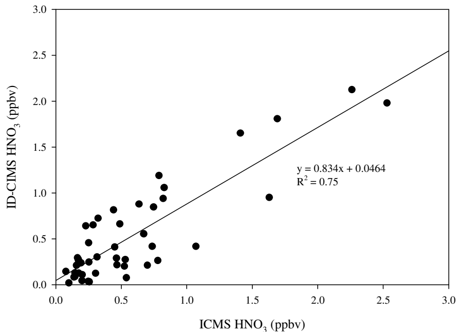
Fig. 10. Inter-comparison between the ID-CIMS and ICMS based on 45 overlapping data points collected from 8 to 29 March 2006.
