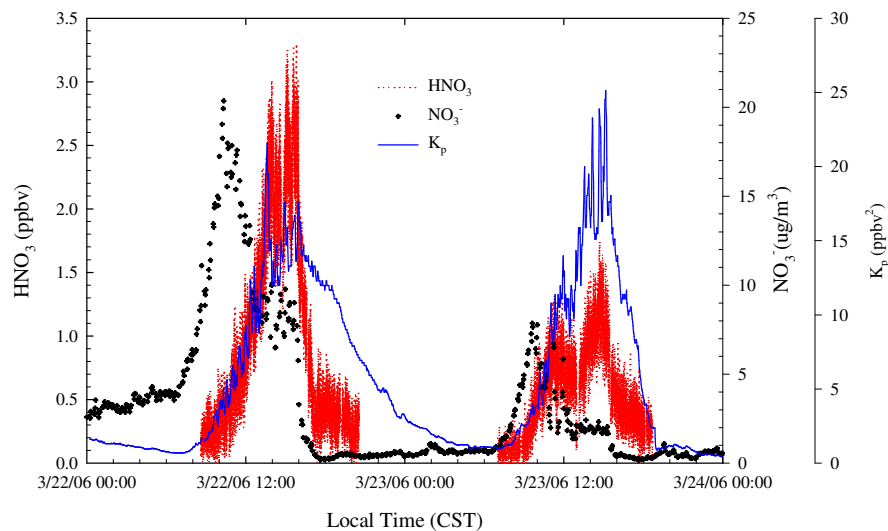
Fig. 8. Gaseous \text{HNO}_3 , aerosol nitrate ( \text{NO}_3^- ), and the calculated dissociation constant K_p of Reaction 18 for 22 and 23 March 2006.
