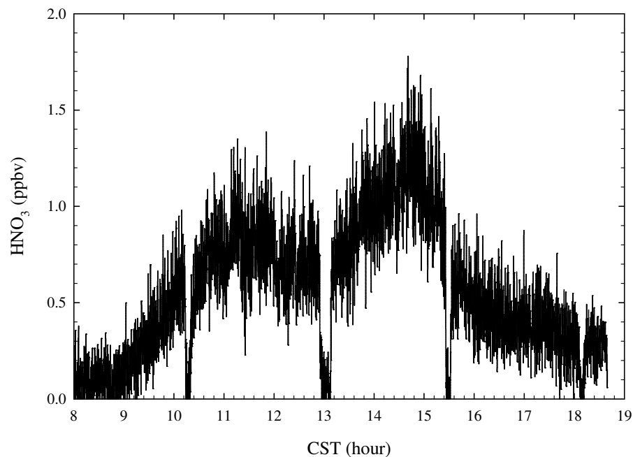
Fig. 6. Diurnal profile of HNO 3 observed on 23 March 2006. Backgrounds were checked at 08:00, 10:15, 13:00, 15:30, and 18:10 CST.
