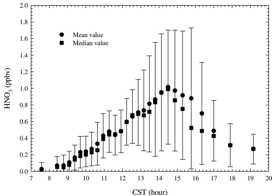
Fig. 7. Averaged HNO 3 diurnal profile during the entire field campaign. Each point is based on 1755 data points and the error bars represent one standard deviation.
