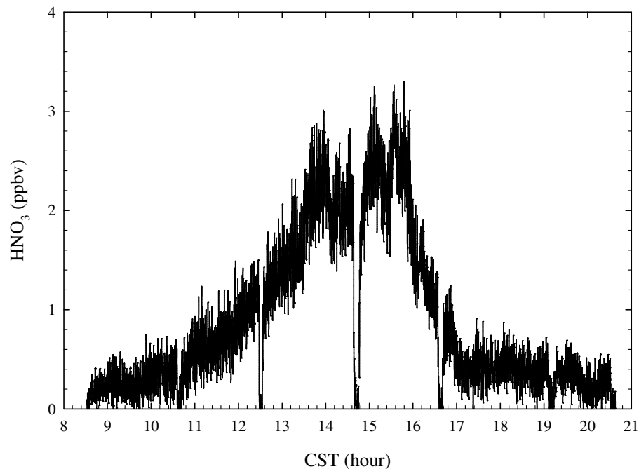
Fig. 5. Diurnal profile of \text{HNO}_3 observed on 22 March 2006. Backgrounds were checked at 08:36, 10:38, 12:30, 14:39, 16:35, 19:20, and 20:35 CST.
