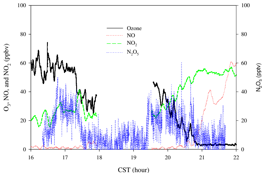
Fig. 9. \text{N}_2\text{O}_5 measured on 26 March. Also shown are plots of \text{NO} , \text{NO}_2 , and \text{O}_3 . The gap in the measurements was due to instrument calibrations.
