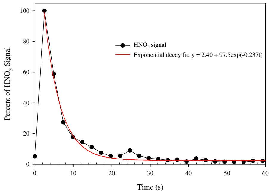
Fig. 4. Spike test of the inlet using a 68 wt % HNO 3 solution exposed to the 12 ft inlet for less than one second. The data was collected at 0.4 Hz.
