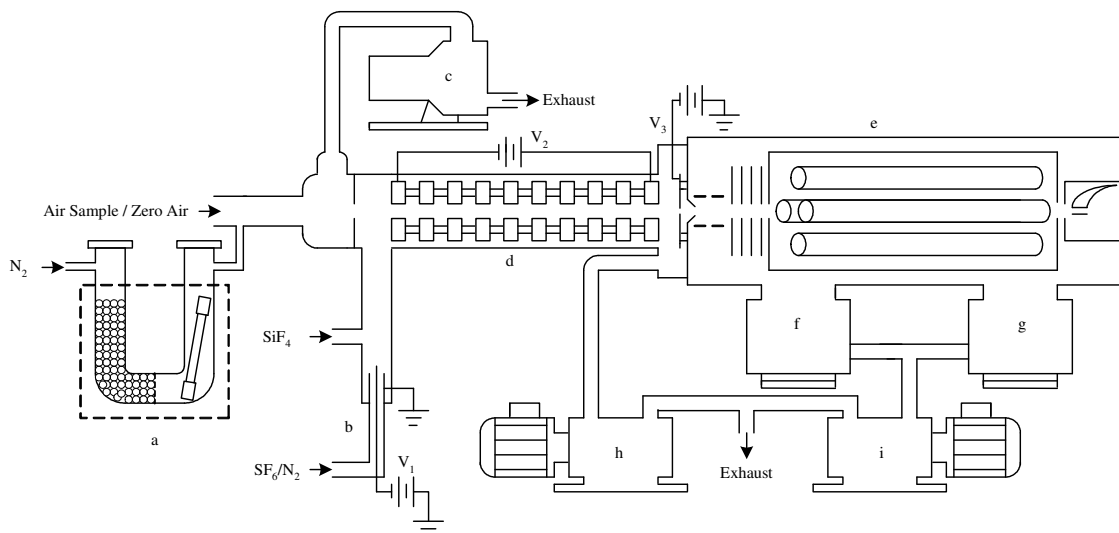
Fig. 1. Schematic diagram of the ID-CIMS: (a) , HNO 3 permeation device; (b) , ion source; (c) , dry scroll pump for air sampling; (d) , 10-ring drift tube; (e) , Extrel 150-QS mass spectrometer; (f) and (g) , Varian TV-551 turbo pumps; (h) , Edwards E2M30 oil pump; (i) , Varian DS402 oil pump.
