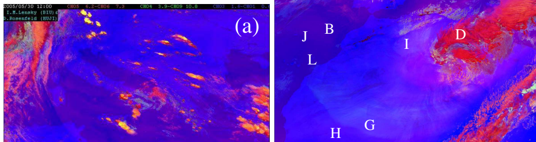
Fig. 9. “Convective Storms” color scheme. (a) Vigorous and severe convective storms appear bright yellow in this color scheme because of the small negative \text{BTDR}_{6.2-7.3} of Cb clouds (high red). The strong updrafts in these clouds produce small ice particles at cloud tops resulting with large \text{BTDR}_{3.9-10.8} (high green). The large absorption at 1.6\ \mu\text{m} by these ice particles keeps the blue very low. Small ice crystals of Cirrus clouds (E in panel (b) ) should not be confused for vigorous convection (a).
