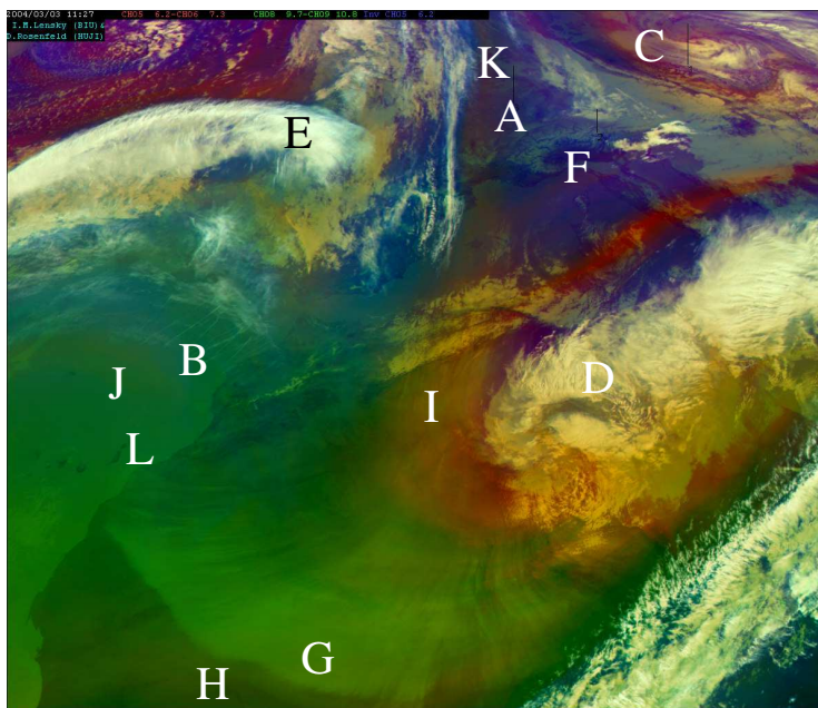
Fig. 15. In the “Air Mass” color scheme, rich ozone polar air mass will have large negative \text{BTDR}_{9.7-10.8} (bluish), while low ozone tropical air mass will have small negative \text{BTDR}_{9.7-10.8} (greenish).
