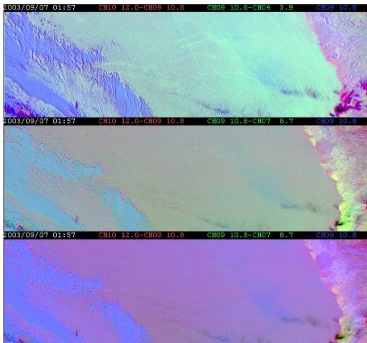
Fig. 14. The 3.9\ \mu\text{m} channel in the “Night Microphysical” color scheme (upper panel) is the most sensitive channel to cloud microphysics. This is demonstrated by ship tracks, which are not seen in the “Day and Night” color scheme (middle panel) or the “Dust” color scheme (lower panel).
