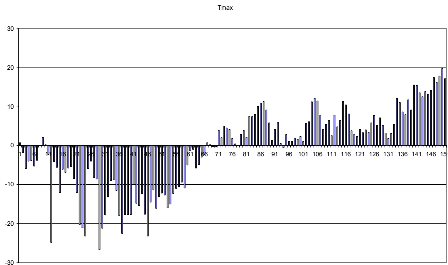
Fig. 7. Air temperature maximum showing the big jump, the “springthaw”.
