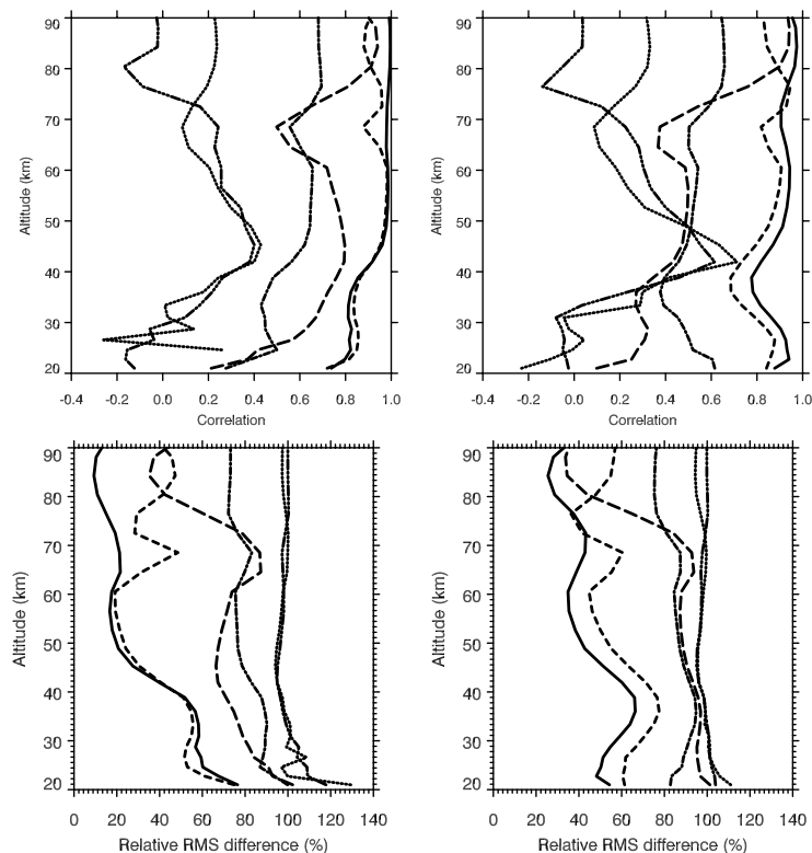
Fig. 5. Temperature: Vertical profiles of the correlation (upper row) and relative RMS difference (lower row) of daily variations of the temperature for SUSIM (left column) and SOLSTICE (right column) with different proxies: Ly- \alpha (long dashed line), 205 nm (dashed line), LYRA (solid line), TSI (dash-dot-dot-dot line), F10.7 (dash-dot line), and NMD (dotted line).
