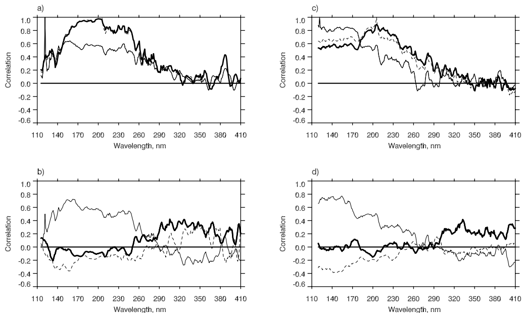
Fig. 1. The correlation of the spectral SUSIM ((a),(b)) and SOLSTICE ((c),(d)) solar irradiance with different proxies: Ly- \alpha (thin line), 205 nm (dashed line), Herz (thick line) ((a), (c)) and TSI (thick line), F10.7 (thin line), and NMD (dashed line) ((b), (d)) for the year 2000.
