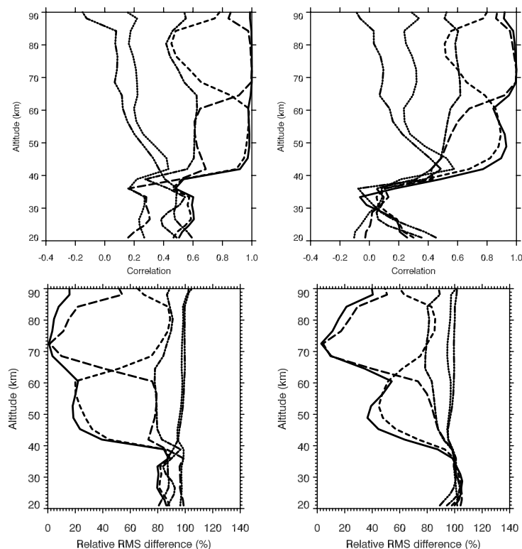
Fig. 3. Hydroxyl: Vertical profiles of the correlation (upper row) and relative RMS difference (lower row) of daily variations of the hydroxyl for SUSIM (left column) and SOLSTICE (right column) with different proxies: Ly- \alpha (long dashed line), 205 nm (dashed line), LYRA (solid line), TSI (dash-dot-dot-dot line), F10.7 (dash-dot line), and NMD (dotted line).
