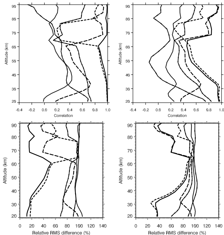
Fig. 4. Ozone: Vertical profiles of the correlation (upper row) and relative RMS difference (lower row) of daily variations of the ozone for SUSIM (left column) and SOLSTICE (right column) with different proxies: Ly- \alpha (long dashed line), 205 nm (dashed line), LYRA (solid line), TSI (dash-dot-dot-dot line), F10.7 (dash-dot line), and NMD (dotted line).
