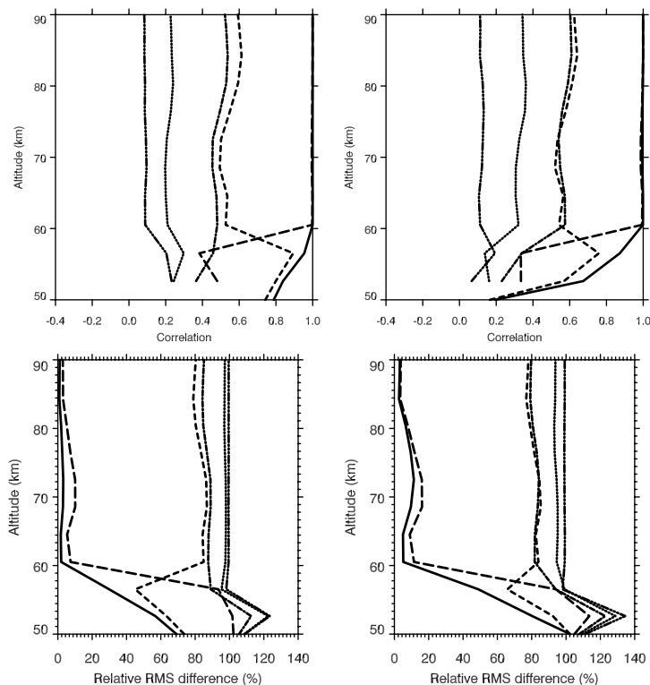
Fig. 2. Positive ions: Vertical profiles of the correlation (upper row) and relative RMS difference (lower row) of daily variations of the total positive ions for SUSIM (left column) and SOLSTICE (right column) with different proxies: Ly- \alpha (long dashed line), 205 nm (dashed line), LYRA (solid line), TSI (dash-dot-dot-dot line), F10.7 (dash-dot line), and NMD (dotted line).
